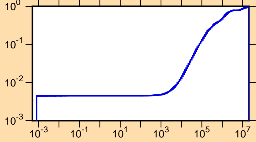
\mu vs. E for ^{152}\text{Sm}(\text{mt251})
