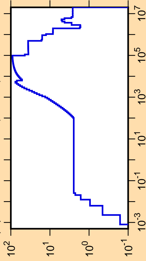
\Delta\mu/\mu vs. E for ^{152}\text{Sm}(\text{mt251})
