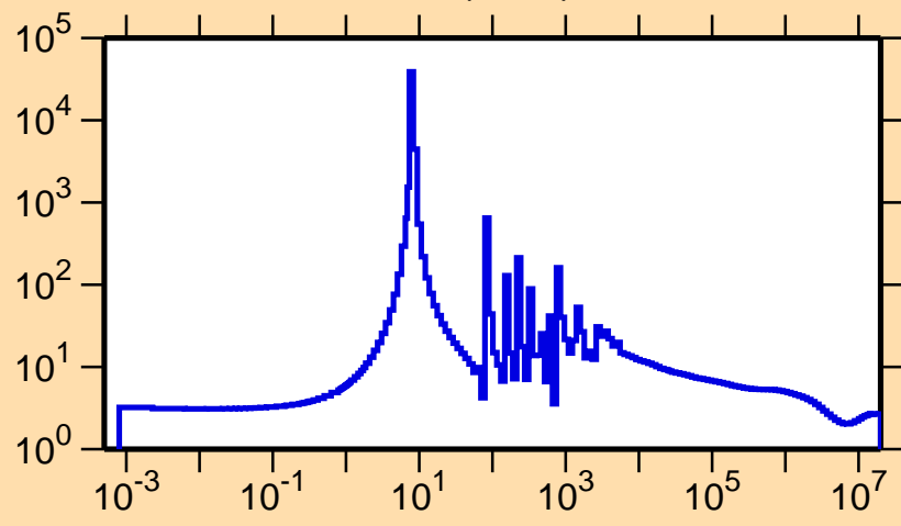
\sigma vs. E for ^{152}\text{Sm}(n,\text{el.})
