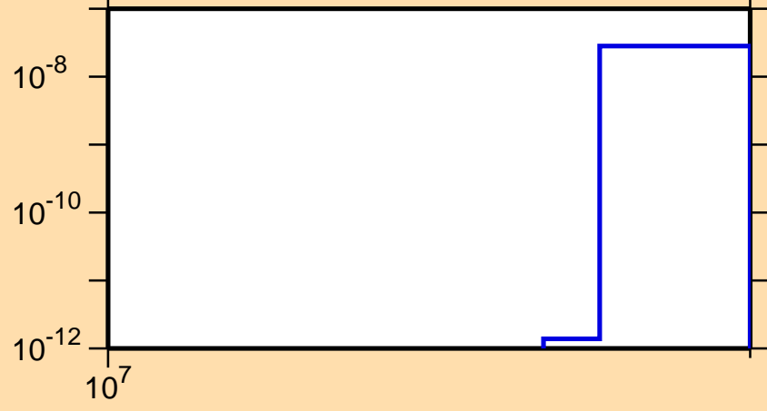
\sigma vs. E for ^{152}\text{Sm}(n,nt)
