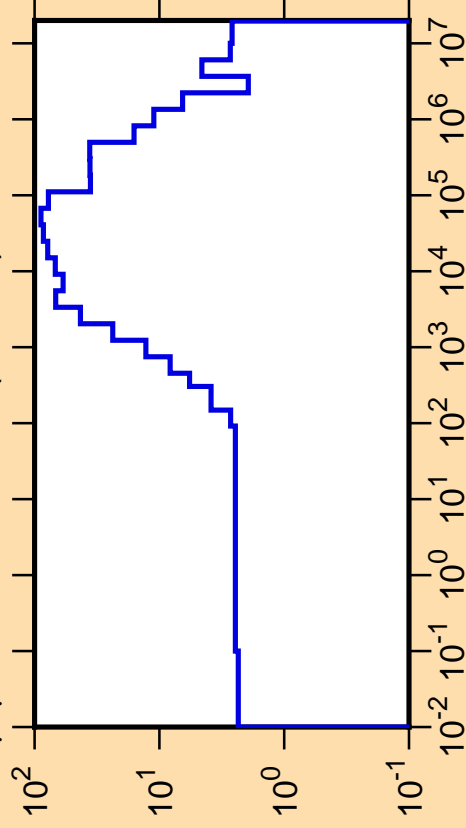
\Delta\mu/\mu vs. E for ^{152}\text{Sm}(\text{mt251})
