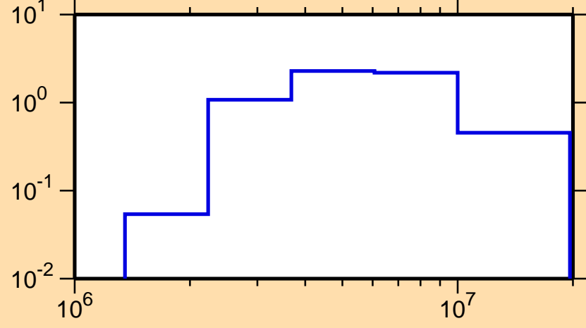
\sigma vs. E for ^{152}\text{Sm}(n,n\text{cont.})
