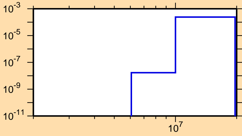
\sigma vs. E for ^{152}\text{Sm}(n,n\alpha)
