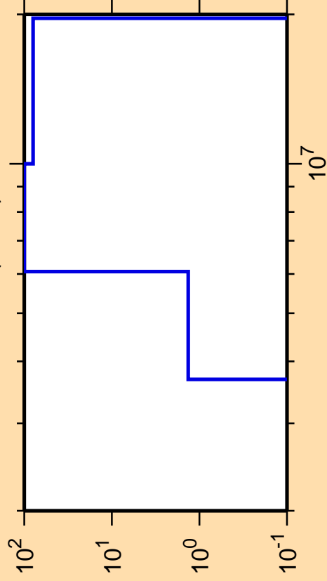
\Delta\sigma/\sigma vs. E for ^{152}\text{Sm}(n,n\alpha)
