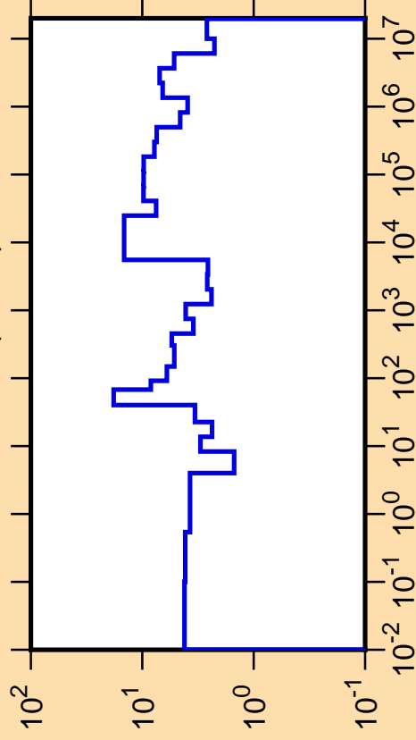
\Delta\sigma/\sigma vs. E for ^{152}\text{Sm}(n,\text{tot.})
