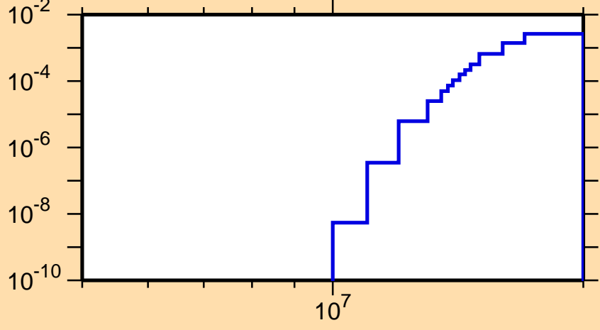
\sigma vs. E for ^{153}\text{Sm}(n,d)
