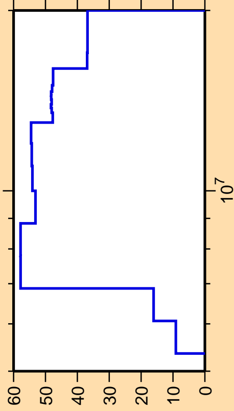
\Delta\sigma/\sigma vs. E for ^{153}\text{Sm}(n,n\text{cont.})
