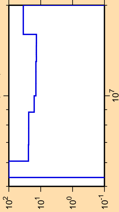
\Delta\sigma/\sigma vs. E for ^{153}\text{Sm}(n,2n)
