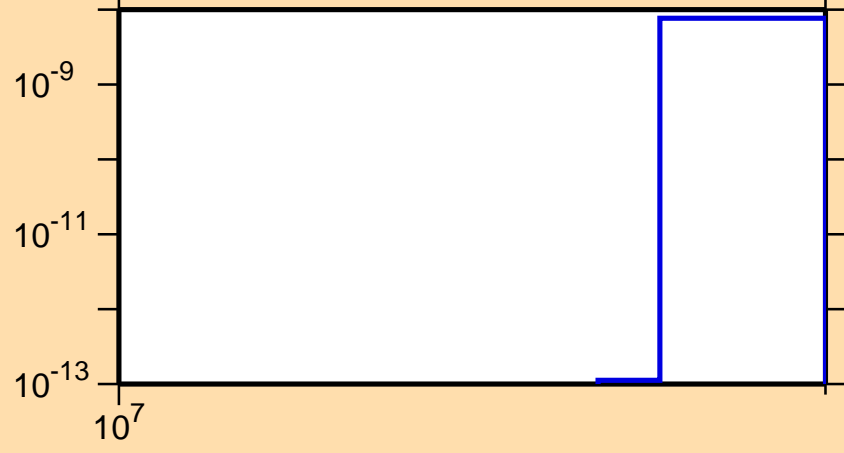
\sigma vs. E for ^{153}\text{Sm}(n,nt)
