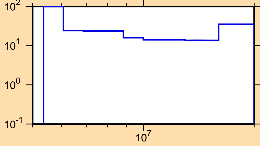
\Delta\sigma/\sigma vs. E for ^{153}\text{Sm}(n,2n)
