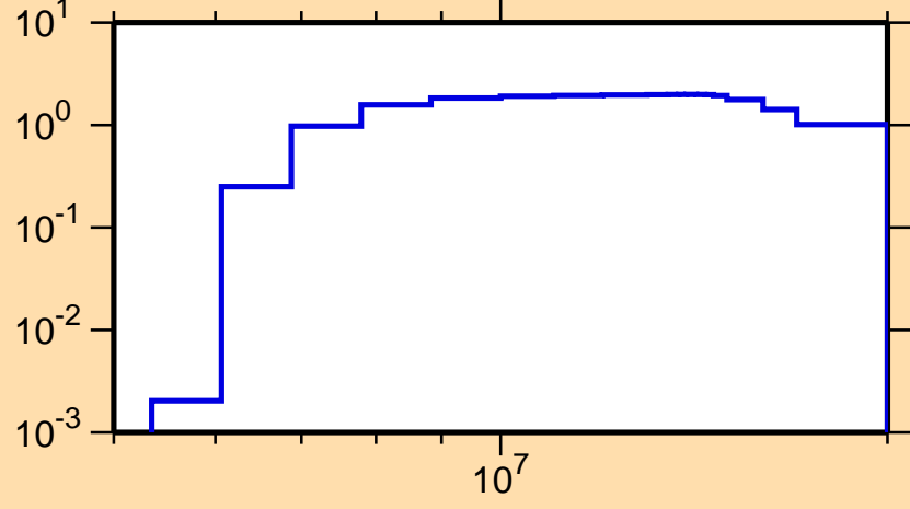
\sigma vs. E for ^{153}\text{Sm}(n,2n)
