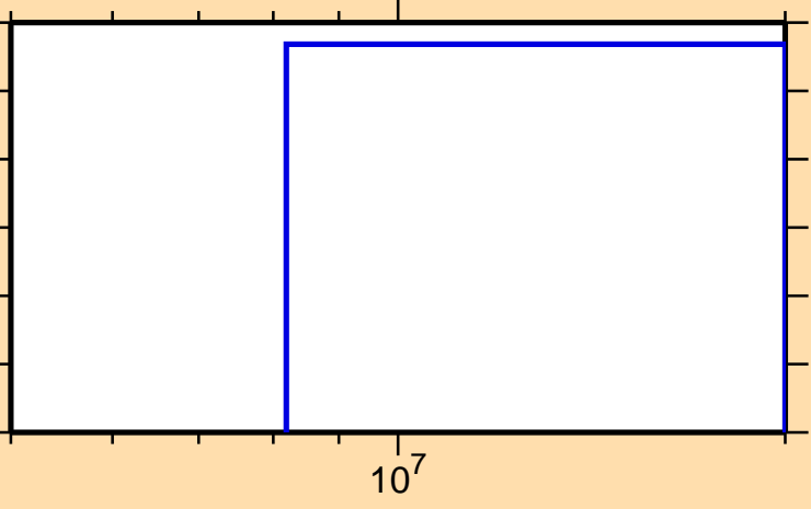
\sigma vs. E for ^{153}\text{Sm}(n,\text{nd})
