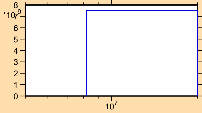
\sigma vs. E for ^{153}\text{Sm}(n,2n\alpha)
