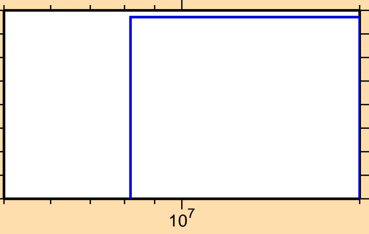
\sigma vs. E for ^{153}\text{Sm}(n,np)
