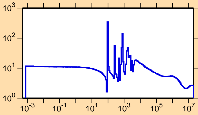
\sigma vs. E for ^{154}\text{Sm}(n,\text{el.})
