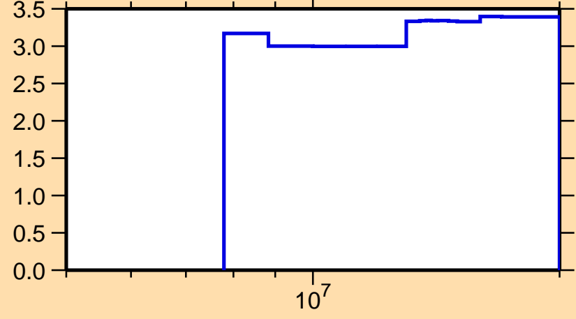
\Delta\sigma/\sigma vs. E for ^{154}\text{Sm}(n,\text{nonel.})
