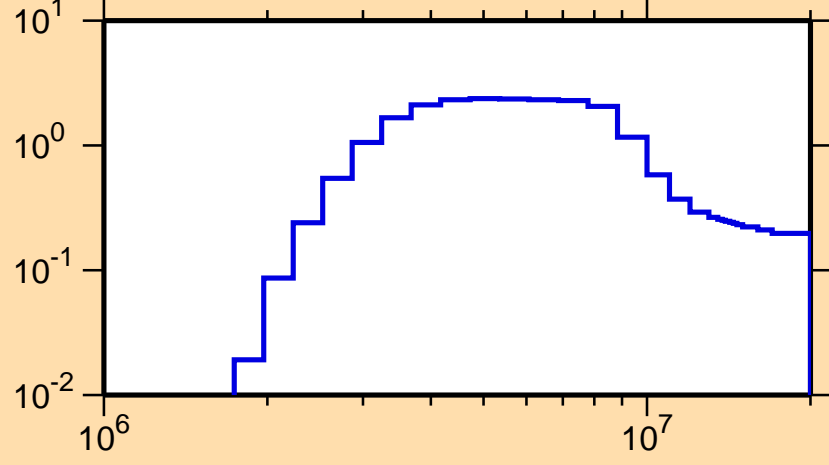
\sigma vs. E for ^{154}\text{Sm}(n,n\text{cont.})
