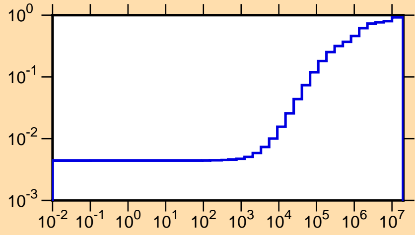
\mu vs. E for ^{154}\text{Sm}(\text{mt251})
