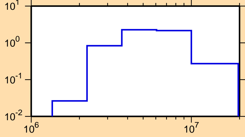
\sigma vs. E for ^{154}\text{Sm}(n,n\text{cont.})
