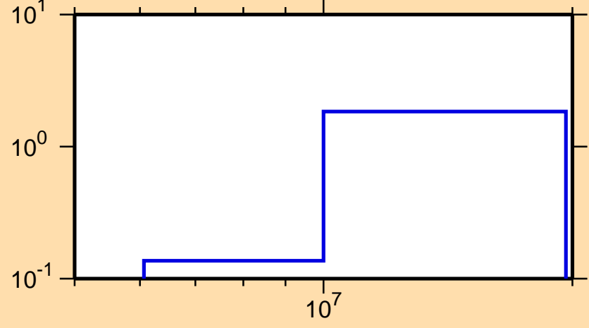
\sigma vs. E for ^{154}\text{Sm}(n,2n)
