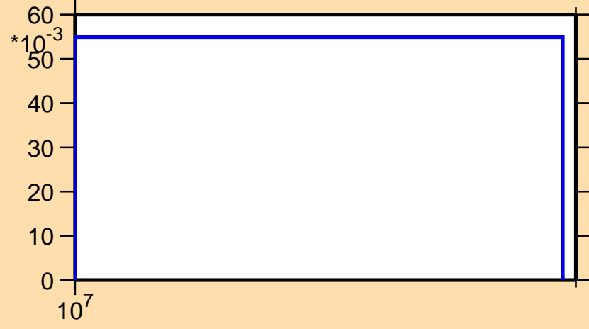
\sigma vs. E for ^{154}\text{Sm}(n,3n)
