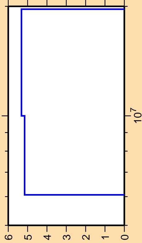
\Delta\sigma/\sigma vs. E for ^{154}\text{Sm}(n,2n)
