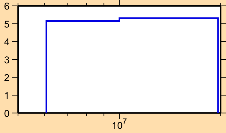
\Delta\sigma/\sigma vs. E for ^{154}\text{Sm}(n,2n)
