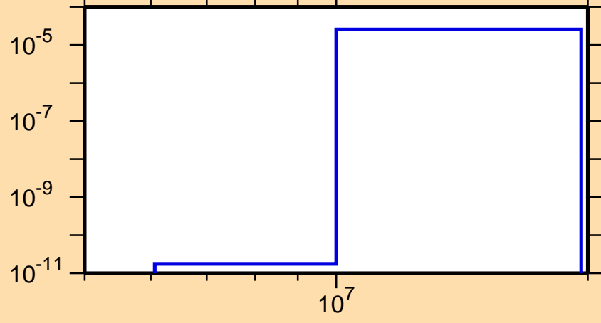
\sigma vs. E for ^{154}\text{Sm}(n,n\alpha)
