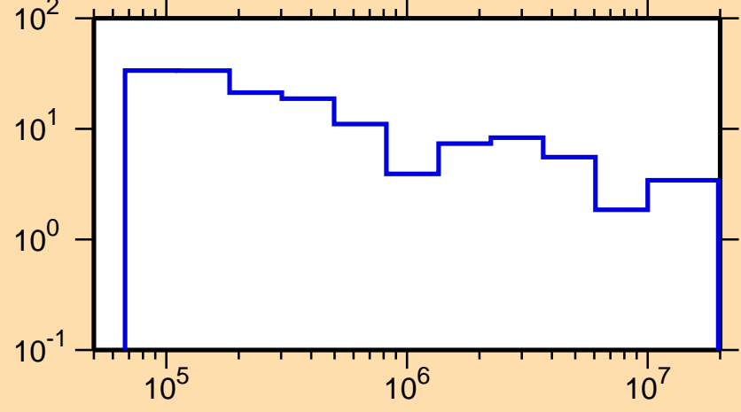
\Delta\sigma/\sigma vs. E for ^{154}\text{Sm}(n,\text{tot.})
