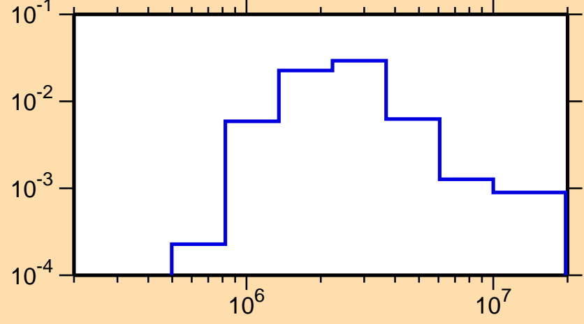
\sigma vs. E for ^{154}\text{Sm}(n,n_3)
