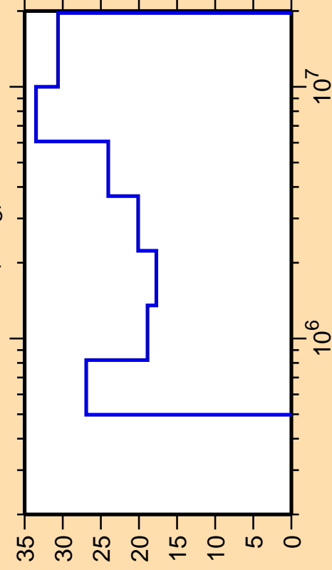
\Delta\sigma/\sigma vs. E for ^{154}\text{Sm}(n,n_3)
