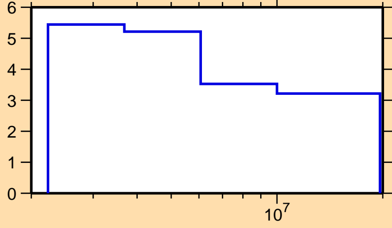
\Delta\sigma/\sigma vs. E for ^{154}\text{Sm}(n,\text{nonel.})
