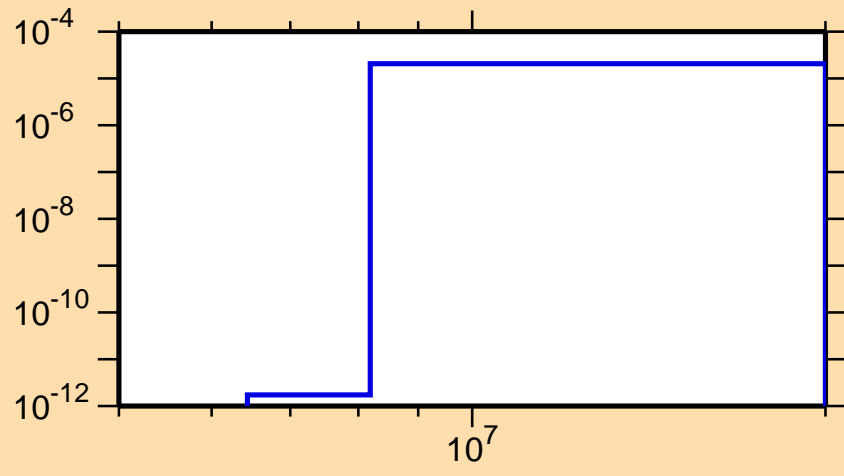
\sigma vs. E for ^{154}\text{Sm}(n,n\alpha)
