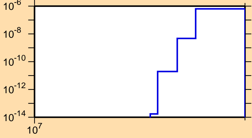
\sigma vs. E for ^{155}\text{Sm}(n,nd)
