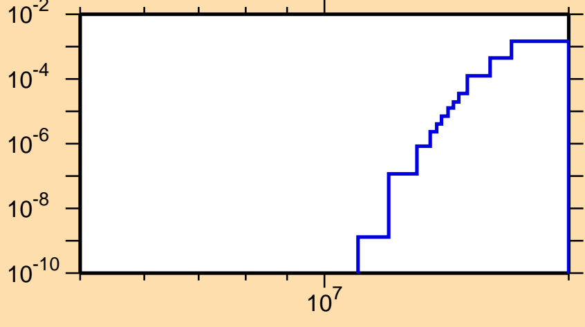
\sigma vs. E for ^{155}\text{Sm}(n,np)
