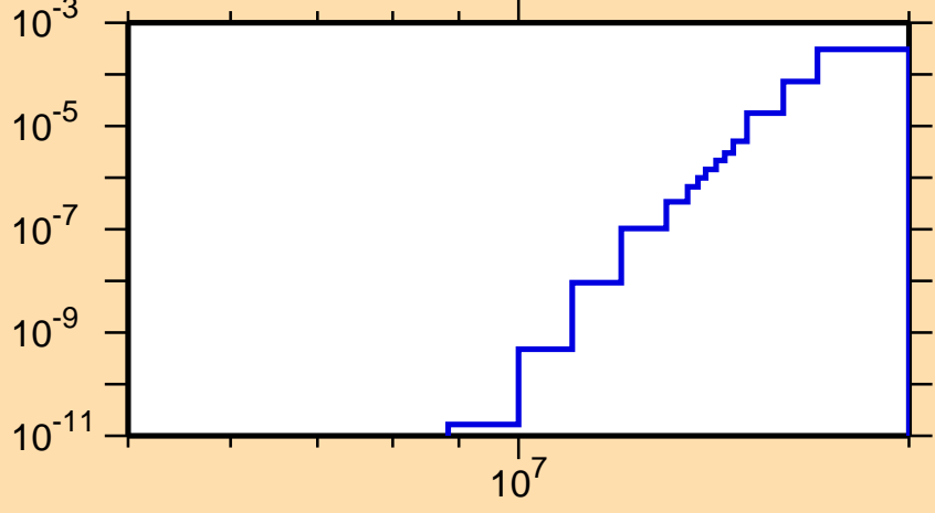
\sigma vs. E for ^{155}\text{Sm}(n,n\alpha)
