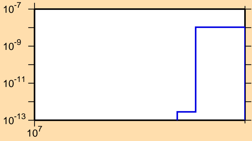
\sigma vs. E for ^{155}\text{Sm}(n,nt)
