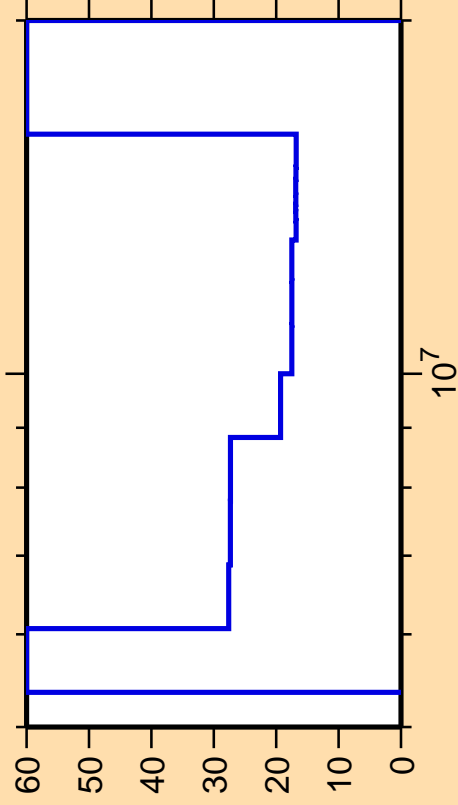
\Delta\sigma/\sigma vs. E for ^{155}\text{Sm}(n,2n)
