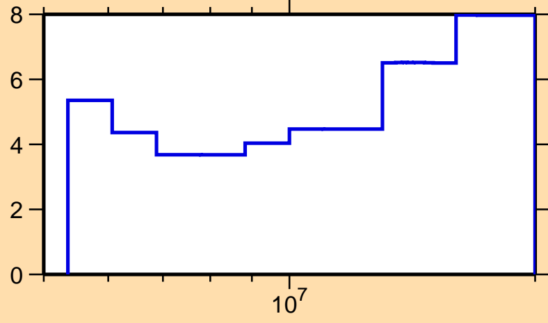
\Delta\sigma/\sigma vs. E for ^{155}\text{Sm}(n,\text{tot.})
