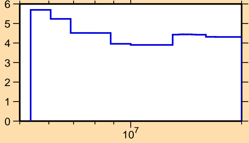
\Delta\sigma/\sigma vs. E for ^{155}\text{Sm}(n,\text{nonel.})
