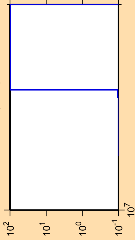
\Delta\sigma/\sigma vs. E for ^{155}\text{Sm}(n,nd)
