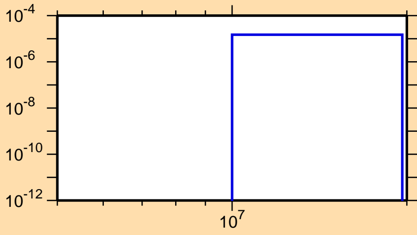
\sigma vs. E for ^{155}\text{Sm}(n,t)
