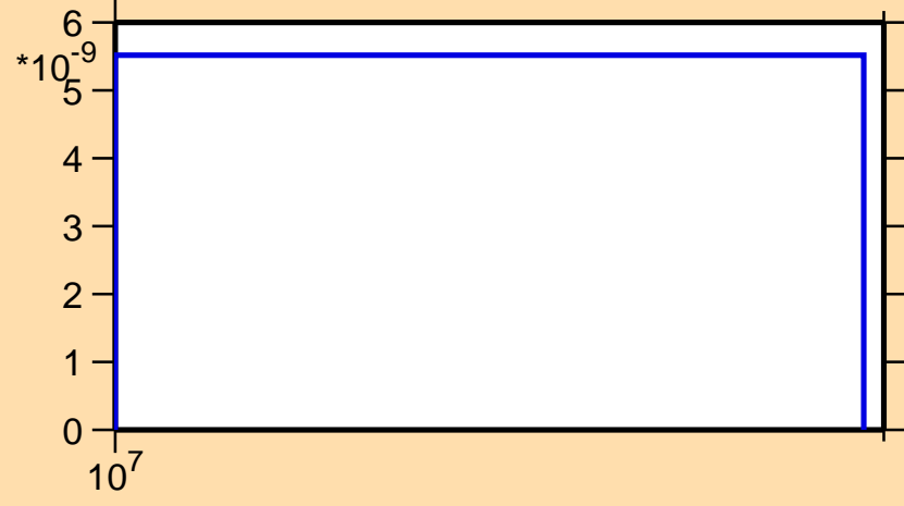
\sigma vs. E for ^{155}\text{Sm}(n,\text{nd})
