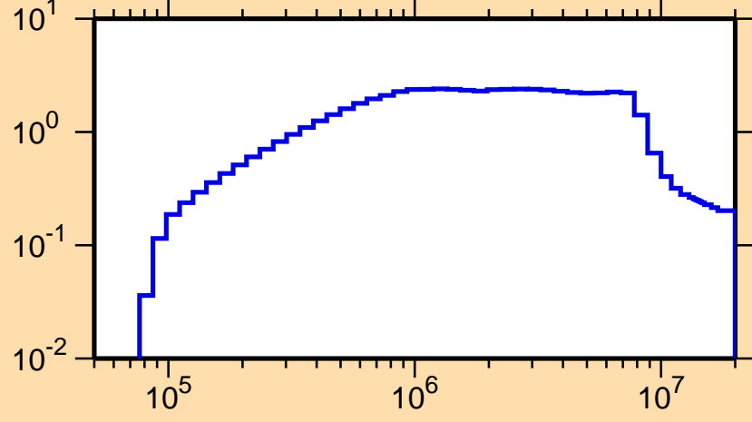
\sigma vs. E for ^{156}\text{Sm}(n,\text{inel.})
