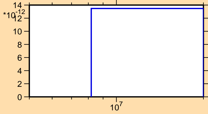
\sigma vs. E for ^{156}\text{Sm}(n,2n\alpha)
