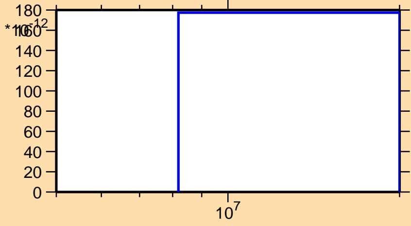
\sigma vs. E for ^{156}\text{Sm}(n,nd)
