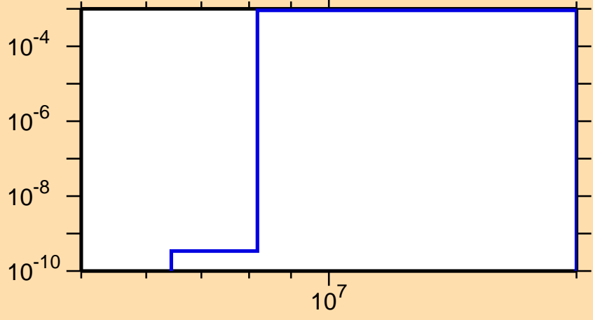
\sigma vs. E for ^{156}\text{Sm}(n,p)
