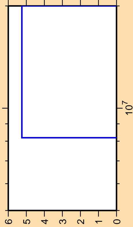
\Delta\sigma/\sigma vs. E for ^{156}\text{Sm}(n,2np)
