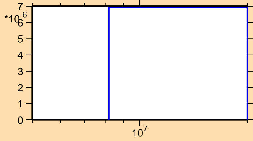
\sigma vs. E for ^{156}\text{Sm}(n,t)
