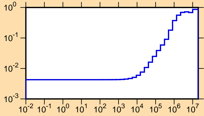
\mu vs. E for ^{158}\text{Sm}(\text{mt251})
