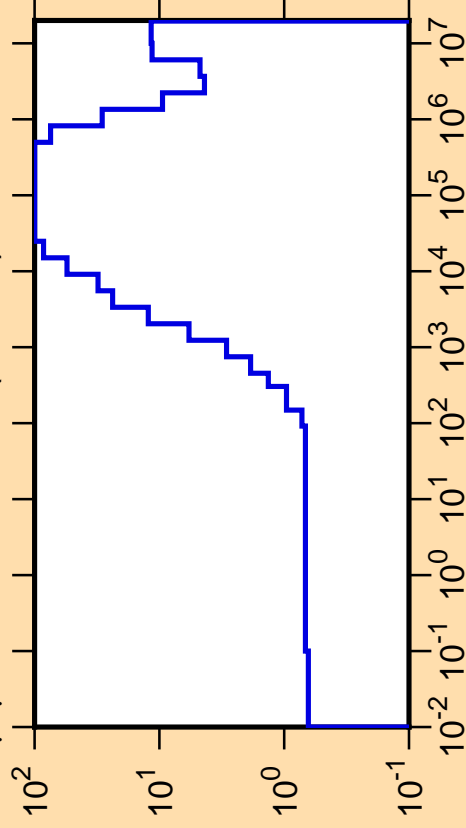
\Delta\mu/\mu vs. E for ^{158}\text{Sm}(\text{mt251})
