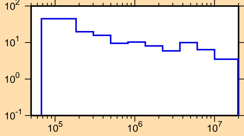
\Delta\sigma/\sigma vs. E for ^{158}\text{Sm}(n,\text{tot.})
