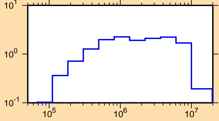
\sigma vs. E for ^{158}\text{Sm}(n,\text{inel.})
