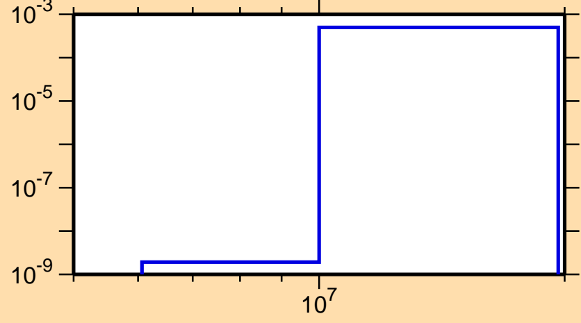
\sigma vs. E for ^{158}\text{Sm}(n,p)
