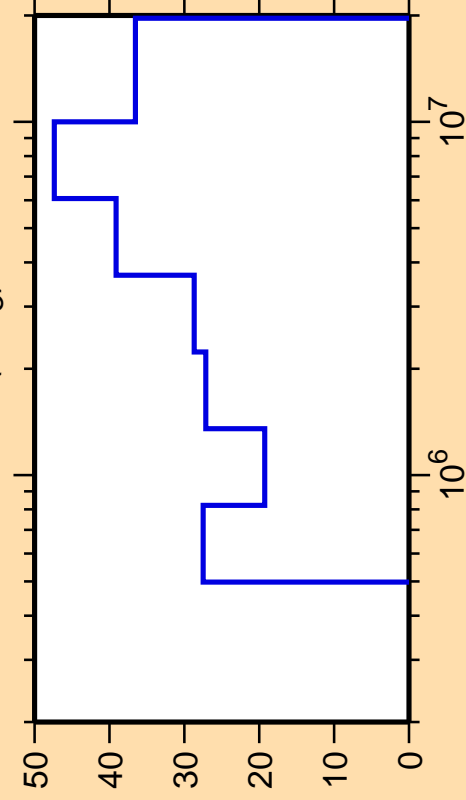
\Delta\sigma/\sigma vs. E for ^{158}\text{Sm}(n,n_3)
