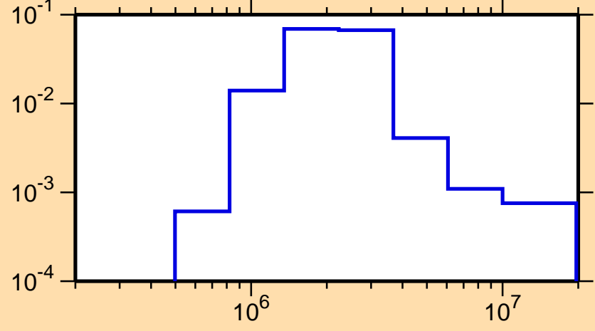
\sigma vs. E for ^{158}\text{Sm}(n,n_3)
