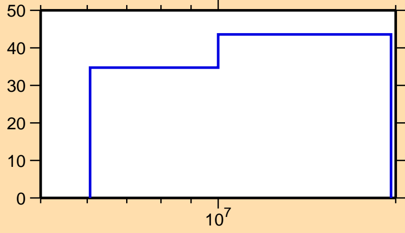
\Delta\sigma/\sigma vs. E for ^{158}\text{Sm}(n,ncont.)
