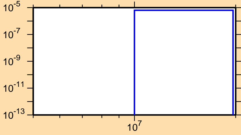
\sigma vs. E for ^{158}\text{Sm}(n,t)
