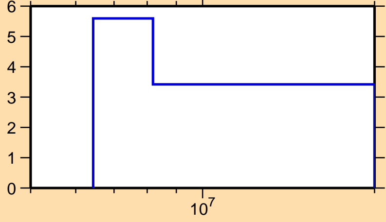
\Delta\sigma/\sigma vs. E for ^{158}\text{Sm}(n,\text{tot.})
