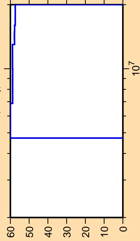
\Delta\sigma/\sigma vs. E for ^{159}\text{Sm}(n,n_1)
