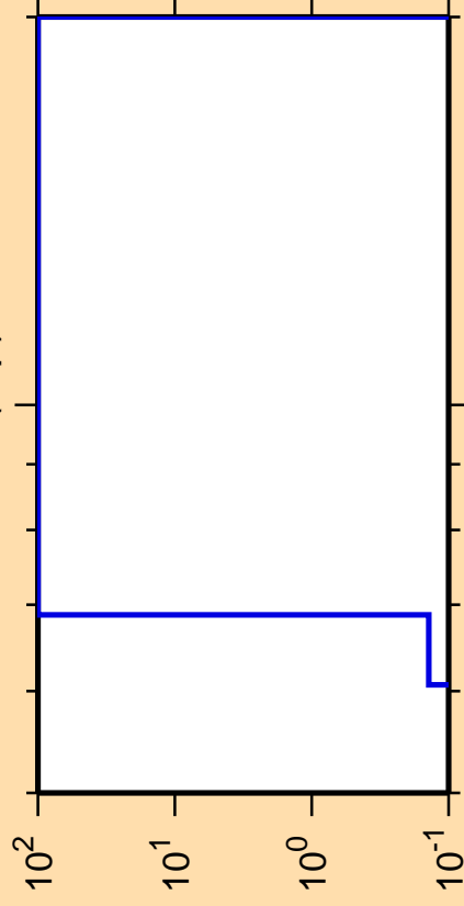
\Delta\sigma/\sigma vs. E for ^{159}\text{Sm}(n,p)
