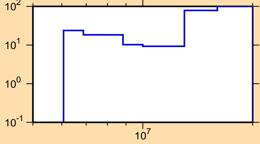
\Delta\sigma/\sigma vs. E for ^{159}\text{Sm}(n,2n)
