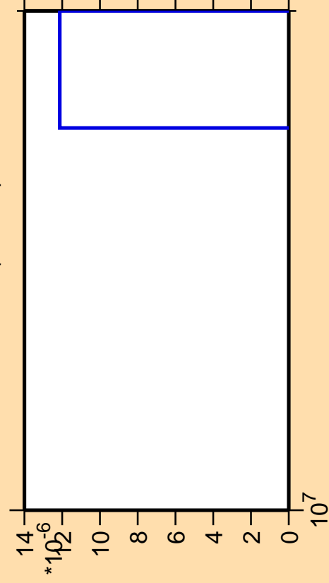
\Delta\sigma/\sigma vs. E for ^{159}\text{Sm} (mt 11)
