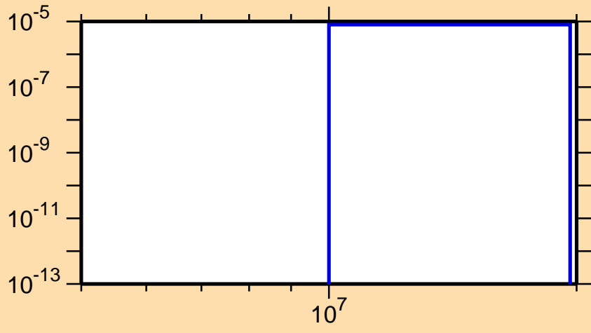
\sigma vs. E for ^{159}\text{Sm}(n,t)
