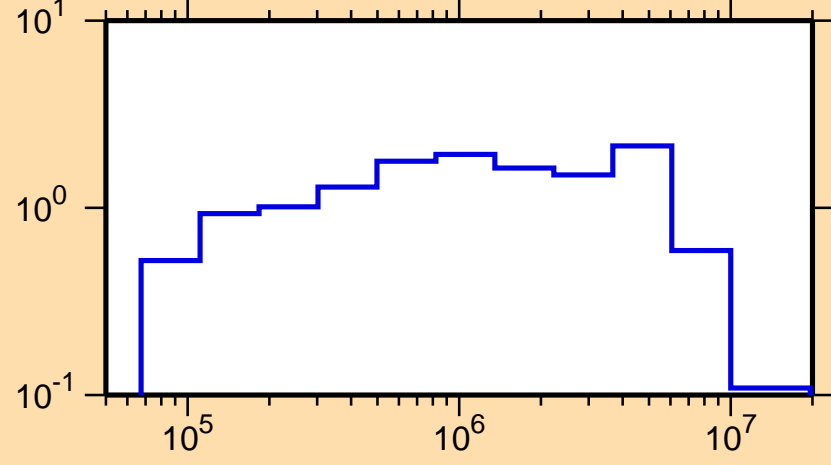
\sigma vs. E for ^{159}\text{Sm}(n,\text{inel.})
