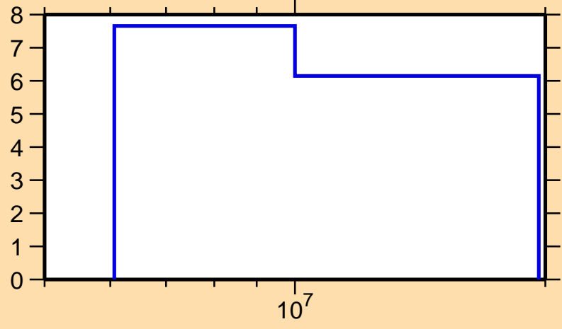
\Delta\sigma/\sigma vs. E for ^{159}\text{Sm}(n,\text{nonel.})
