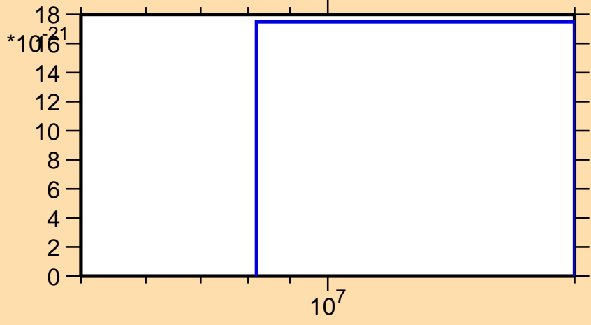
\sigma vs. E for ^{159}\text{Sm}(\text{mt } 11)
