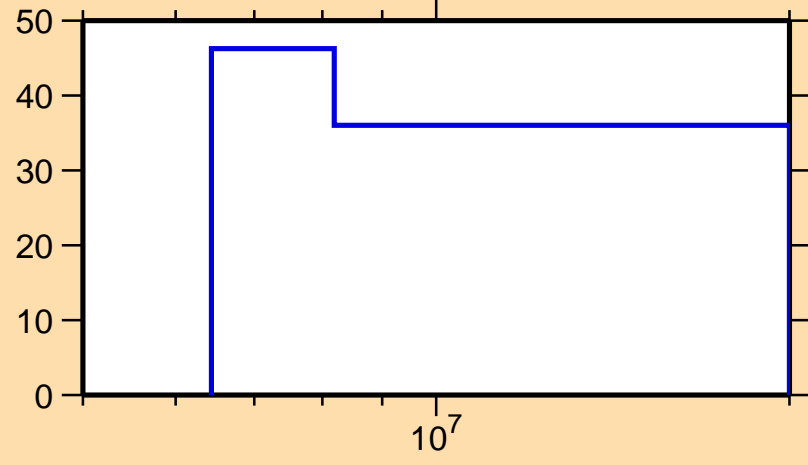
\Delta\sigma/\sigma vs. E for ^{159}\text{Sm}(n,el.)
