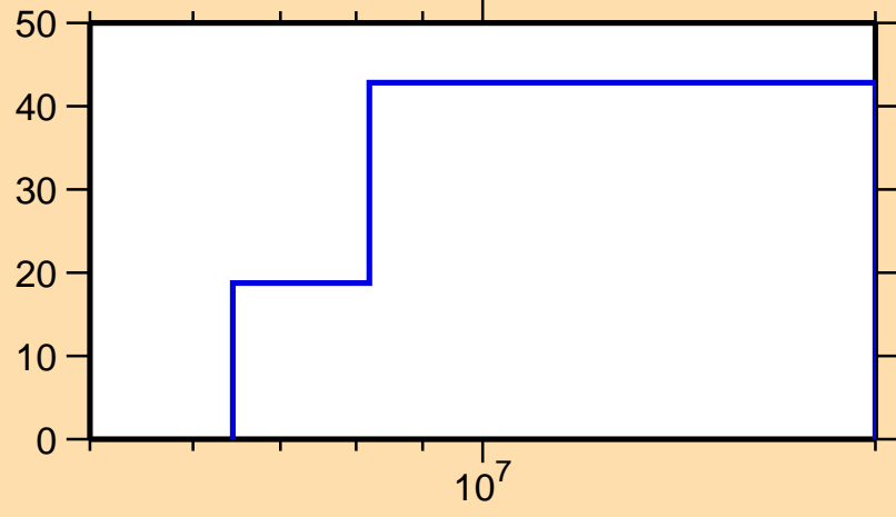
\Delta\sigma/\sigma vs. E for ^{159}\text{Sm}(n,2n)
