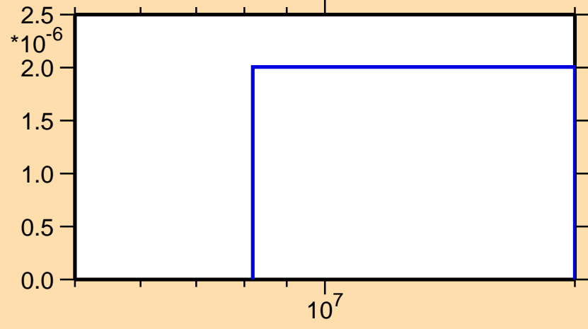
\sigma vs. E for ^{159}\text{Sm}(n,n\alpha)
