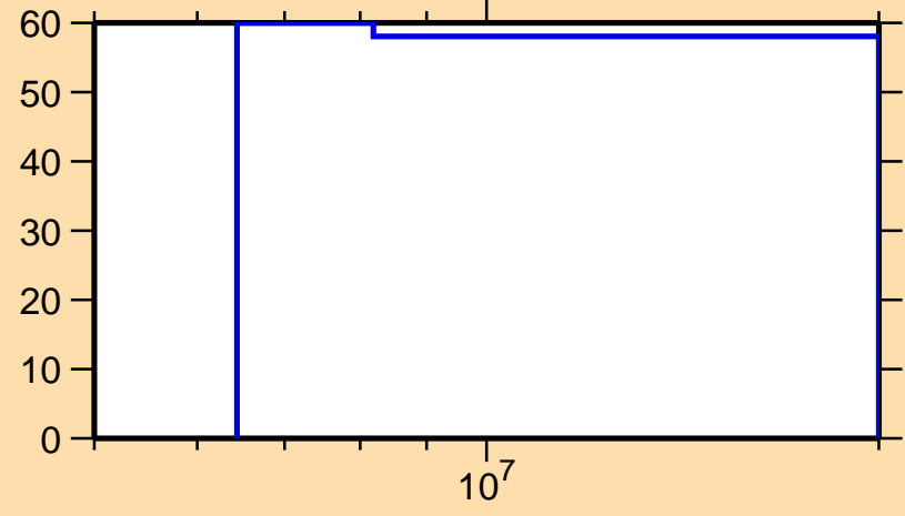
\Delta\sigma/\sigma vs. E for ^{159}\text{Sm}(n,ncont.)
