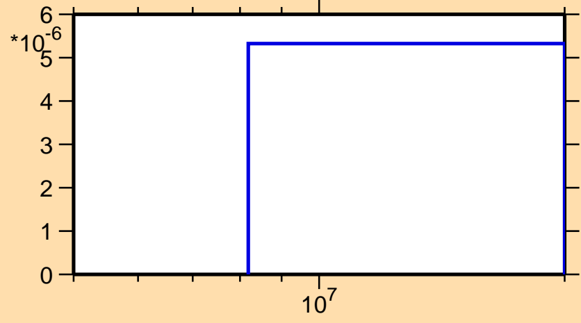
\sigma vs. E for ^{159}\text{Sm}(n,np)
