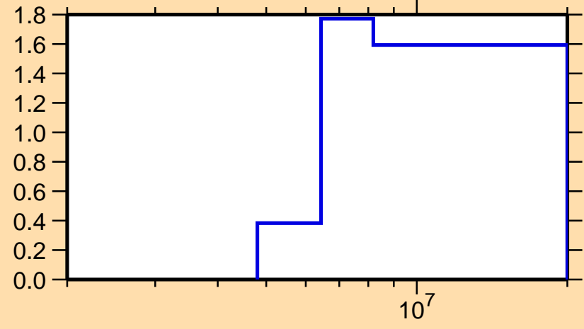
\sigma vs. E for ^{159}\text{Sm}(n,2n)
