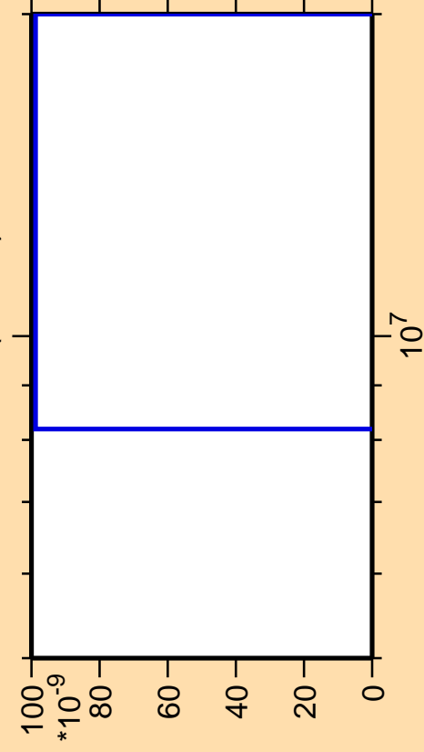
\Delta\sigma/\sigma vs. E for ^{159}\text{Sm}(\text{mt } 11)
