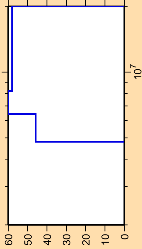
\Delta\sigma/\sigma vs. E for ^{159}\text{Sm}(n,n\text{cont.})
