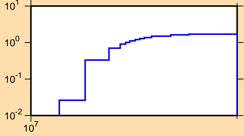
\sigma vs. E for ^{160}\text{Sm}(n,3n)
