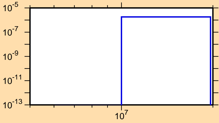
\sigma vs. E for ^{160}\text{Sm}(n,n\alpha)
