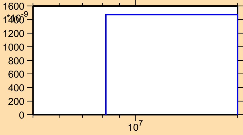
\sigma vs. E for ^{160}\text{Sm}(n,n\alpha)
