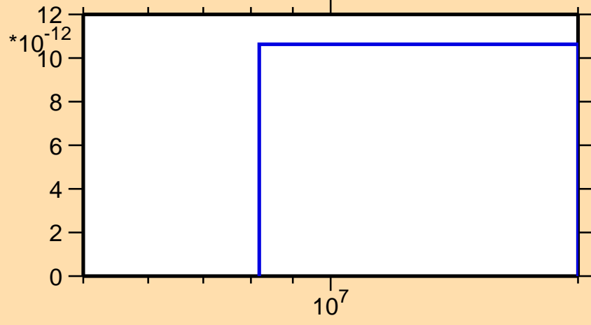
\sigma vs. E for ^{160}\text{Sm}(n,2n\alpha)
