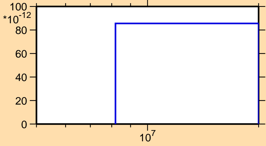
\sigma vs. E for ^{160}\text{Sm}(n,nd)
