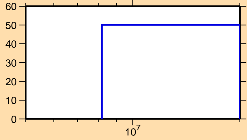
\Delta\sigma/\sigma vs. E for ^{160}\text{Sm}(n,2n)
