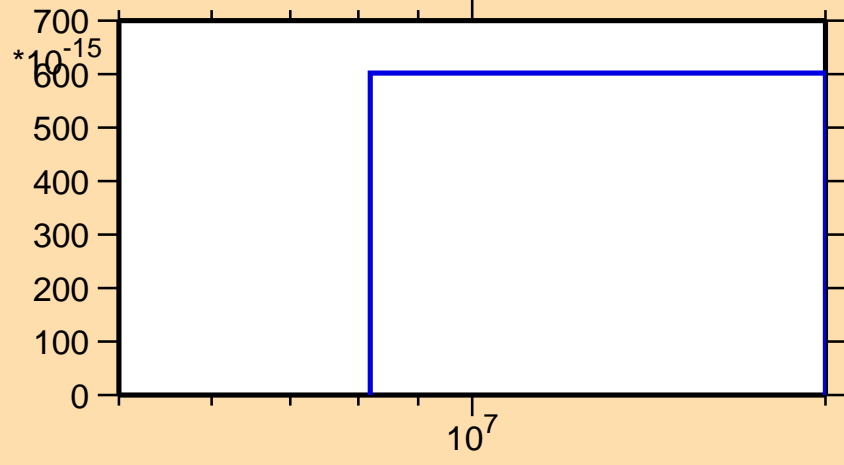
\sigma vs. E for ^{160}\text{Sm}(n,2np)
