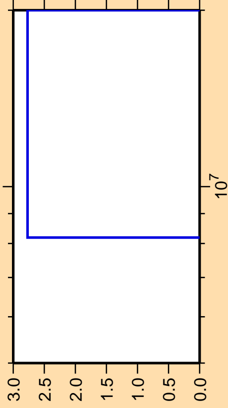
\Delta\sigma/\sigma vs. E for ^{160}\text{Sm}(n,2np)
