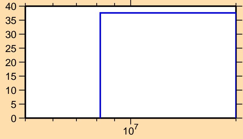
\Delta\sigma/\sigma vs. E for ^{160}\text{Sm}(n,el.)
