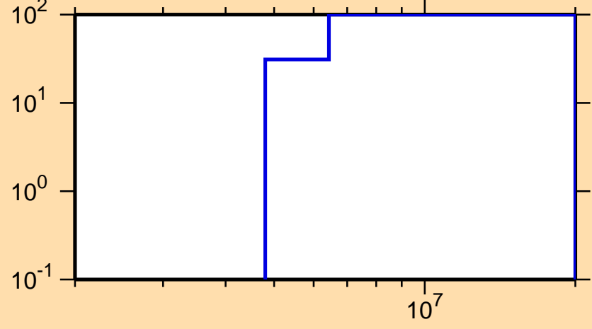
\Delta\sigma/\sigma vs. E for ^{160}\text{Sm}(n,\text{inel.})
