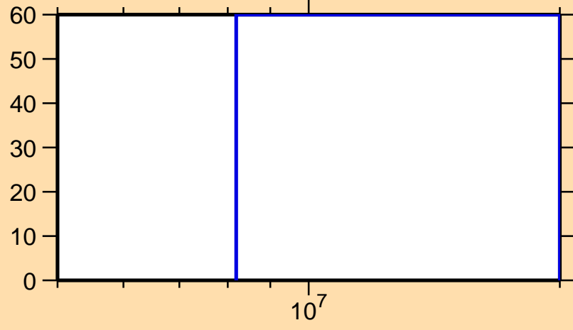
\Delta\sigma/\sigma vs. E for ^{160}\text{Sm}(n,p)
