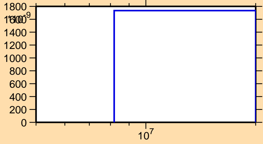
\sigma vs. E for ^{160}\text{Sm}(n,np)
