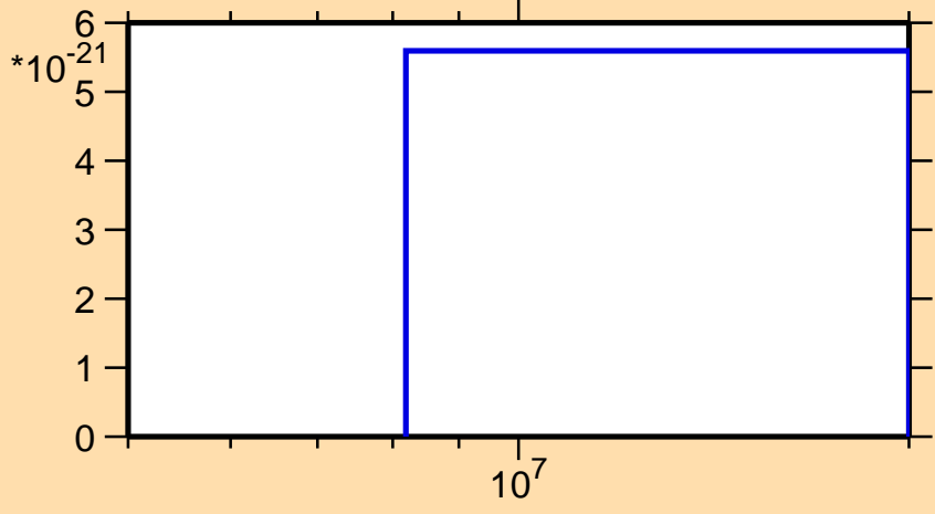
\sigma vs. E for ^{160}\text{Sm}(\text{mt } 11)
