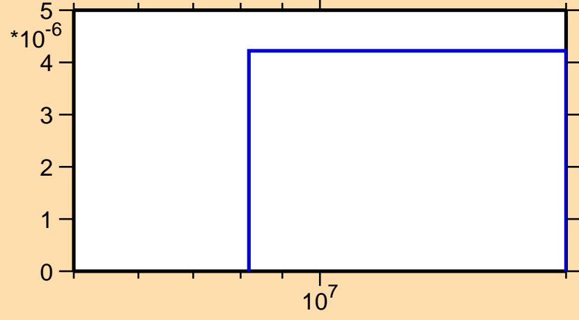
\sigma vs. E for ^{160}\text{Sm}(n,t)
