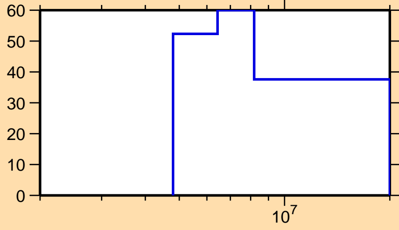
\Delta\sigma/\sigma vs. E for ^{160}\text{Sm}(n,\text{el.})
