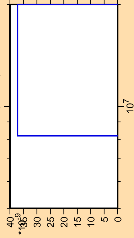
\Delta\sigma/\sigma vs. E for ^{160}\text{Sm}(\text{mt } 11)
