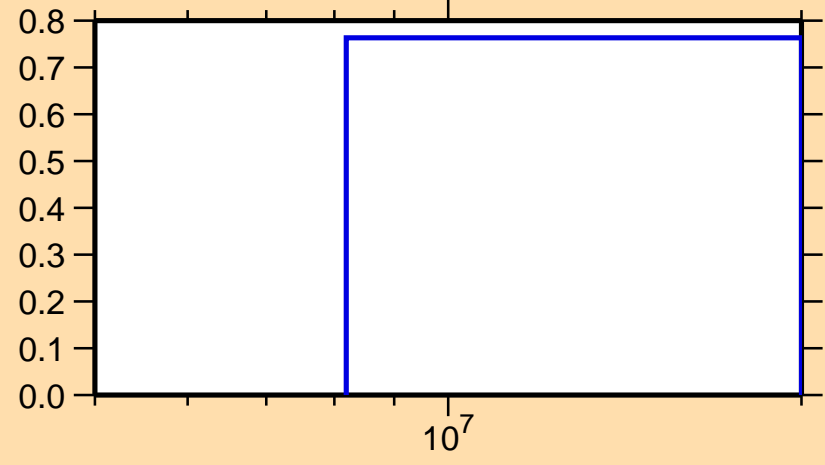
\sigma vs. E for ^{160}\text{Sm}(n,3n)
