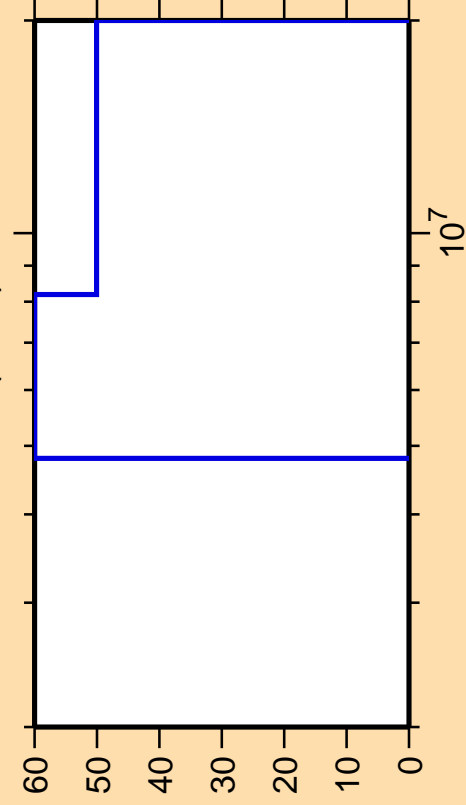
\Delta\sigma/\sigma vs. E for ^{160}\text{Sm}(n,2n)
