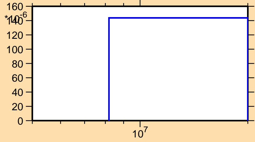
\sigma vs. E for ^{160}\text{Sm}(n,p)
