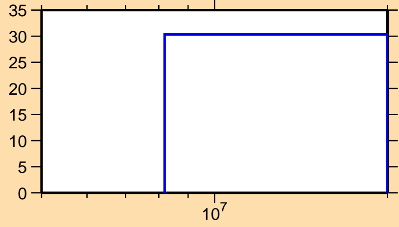
\Delta\sigma/\sigma vs. E for ^{160}\text{Sm}(n,\text{nonel.})
