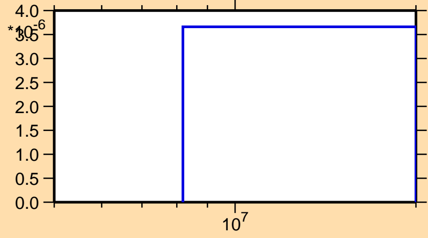
\sigma vs. E for ^{160}\text{Sm}(n,d)
