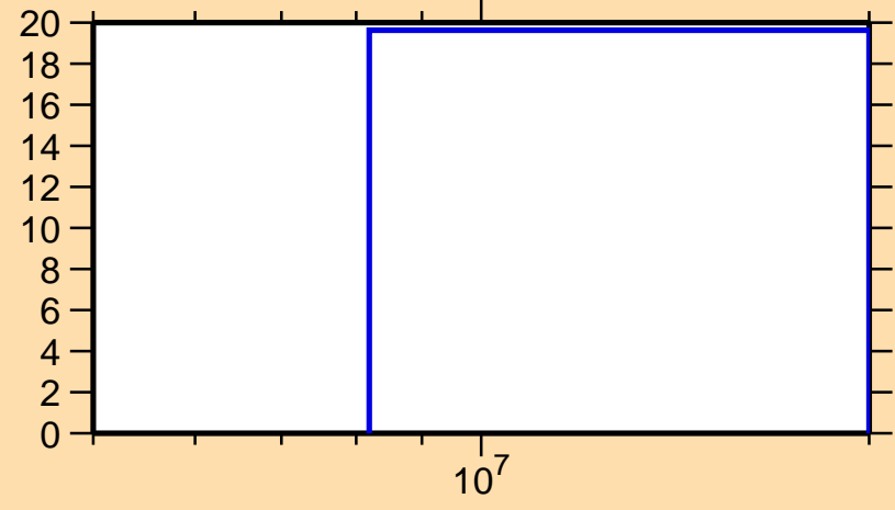
\Delta\sigma/\sigma vs. E for ^{160}\text{Sm}(n,\text{tot.})
