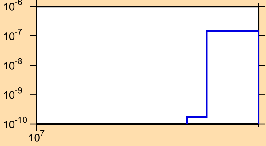
\sigma vs. E for ^{161}\text{Sm}(n,\text{nd})
