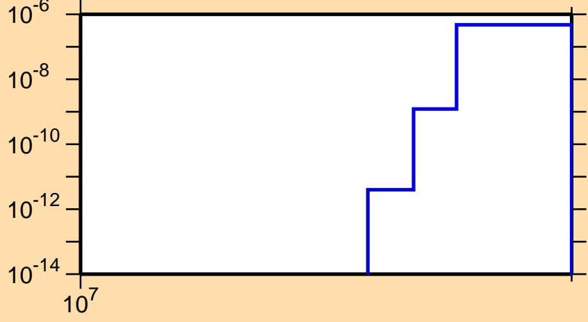
\sigma vs. E for ^{161}\text{Sm}(n,nt)
