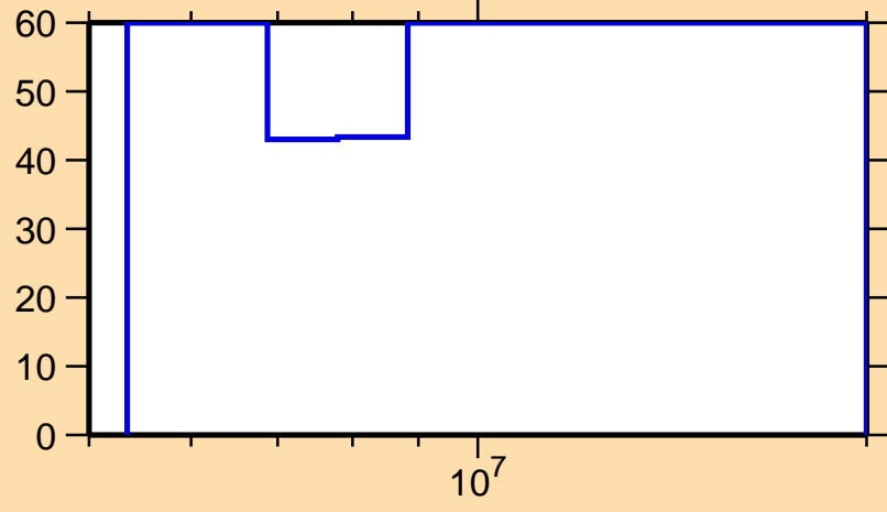
\Delta\sigma/\sigma vs. E for ^{161}\text{Sm}(n,\text{inel.})
