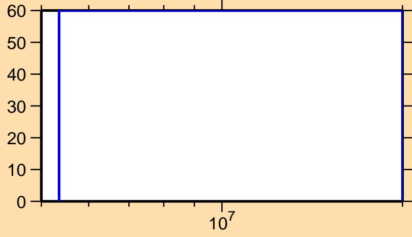
\Delta\sigma/\sigma vs. E for ^{161}\text{Sm}(n,\gamma)
