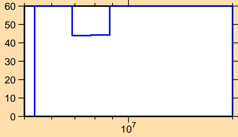
\Delta\sigma/\sigma vs. E for ^{161}\text{Sm}(n,ncont.)
