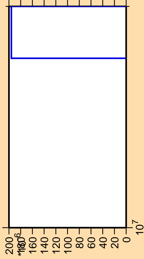
\Delta\sigma/\sigma vs. E for ^{161}\text{Sm} (mt 11)
