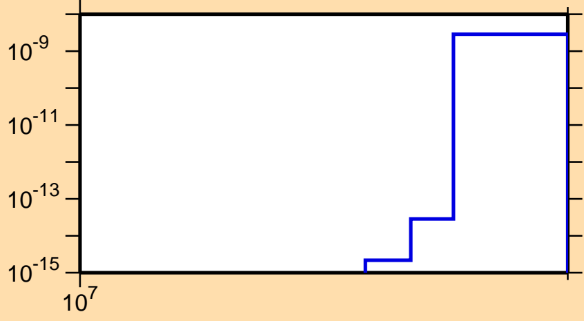
\sigma vs. E for ^{161}\text{Sm}(n,2np)
