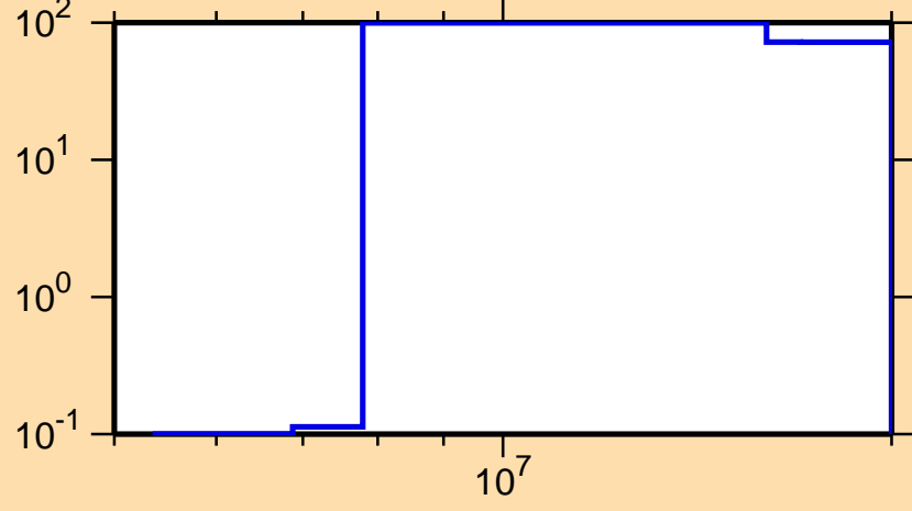
\Delta\sigma/\sigma vs. E for ^{161}\text{Sm}(n,p)
