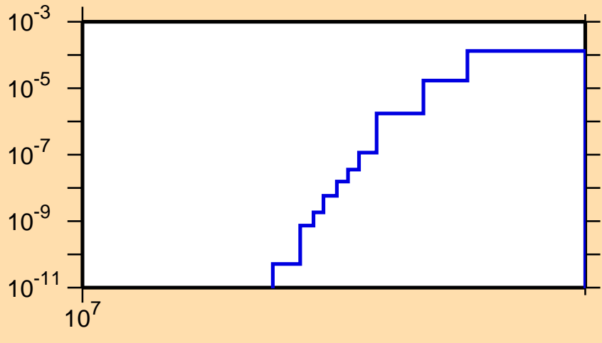
\sigma vs. E for ^{161}\text{Sm}(n,np)
