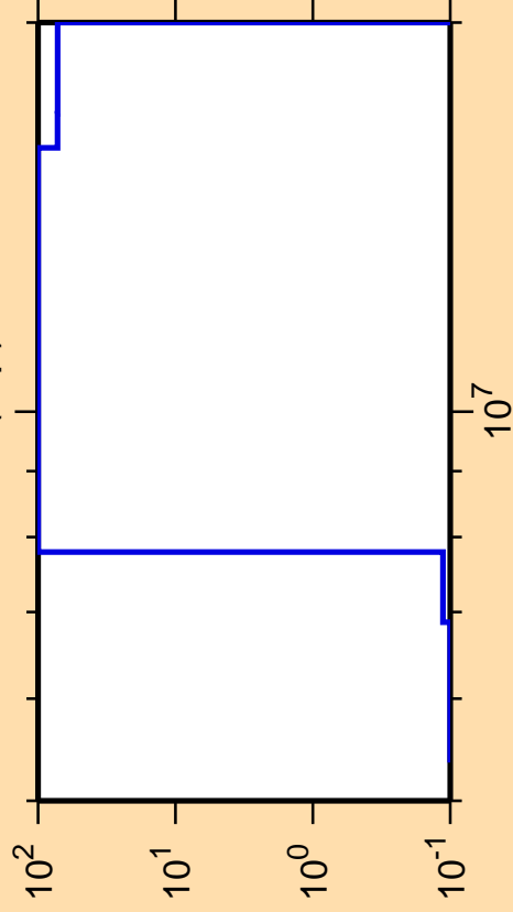
\Delta\sigma/\sigma vs. E for ^{161}\text{Sm}(n,p)
