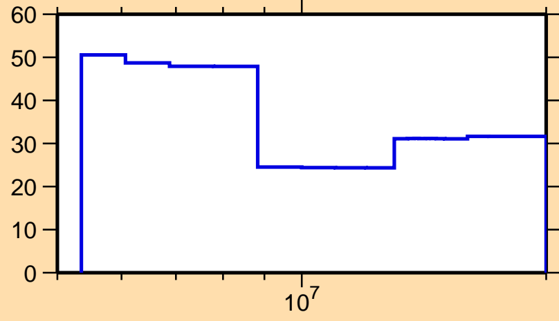
\Delta\sigma/\sigma vs. E for ^{161}\text{Sm}(n,el.)
