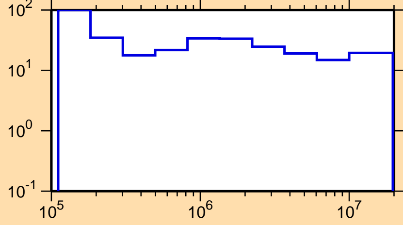
\Delta\sigma/\sigma vs. E for ^{161}\text{Sm}(n,\text{nonel.})
