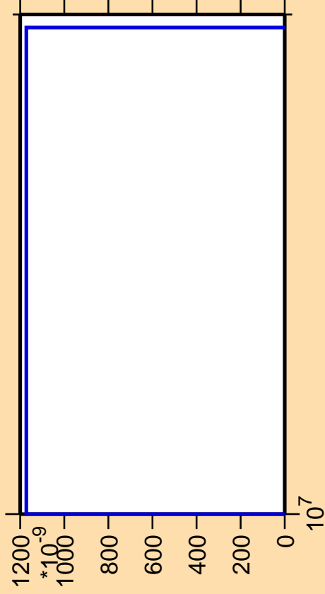
\Delta\sigma/\sigma vs. E for ^{161}\text{Sm}(\text{mt } 11)
