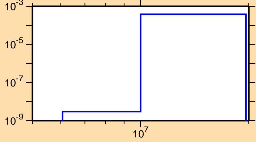
\sigma vs. E for ^{161}\text{Sm}(n,p)
