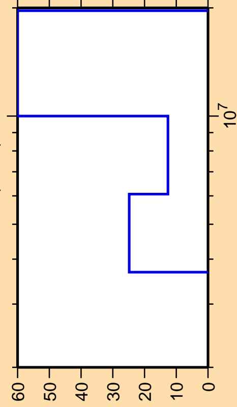
\Delta\sigma/\sigma vs. E for ^{161}\text{Sm}(n,2n)
