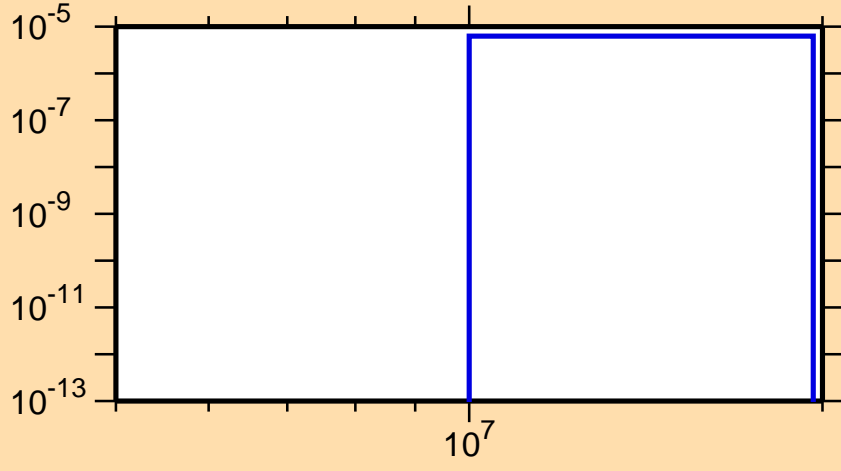
\sigma vs. E for ^{161}\text{Sm}(n,t)
