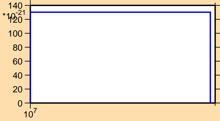
\sigma vs. E for ^{161}\text{Sm}(\text{mt } 11)
