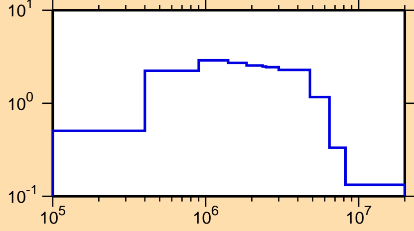
\sigma vs. E for ^{161}\text{Sm}(n,\text{inel.})
