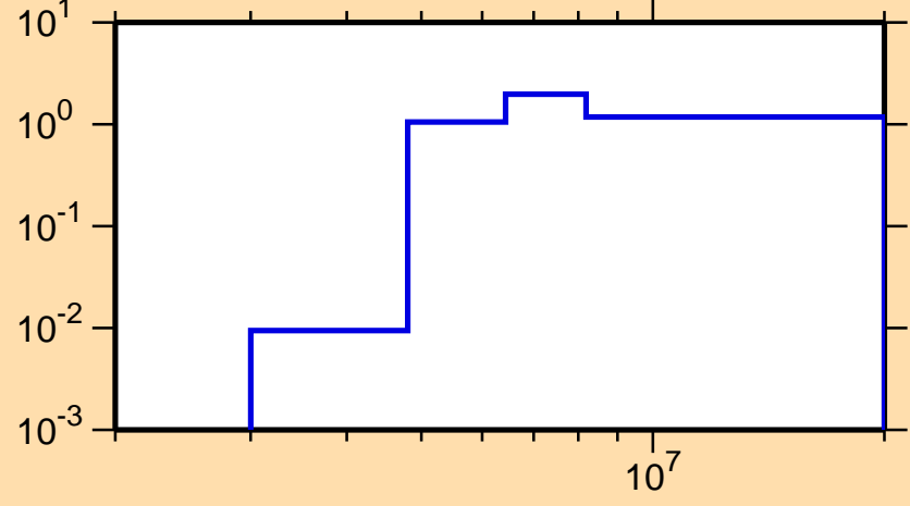
\sigma vs. E for ^{161}\text{Sm}(n,2n)
