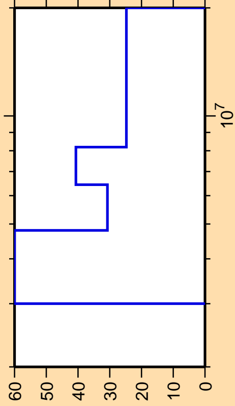
\Delta\sigma/\sigma vs. E for ^{161}\text{Sm}(n,n_1)
