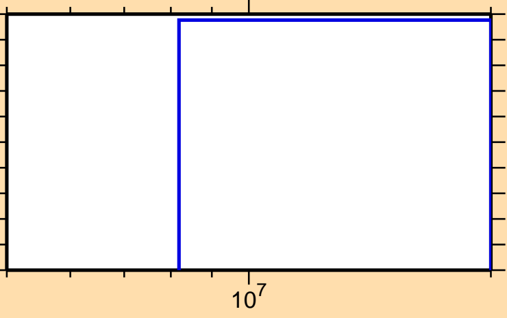
\sigma vs. E for ^{161}\text{Sm}(n,np)
