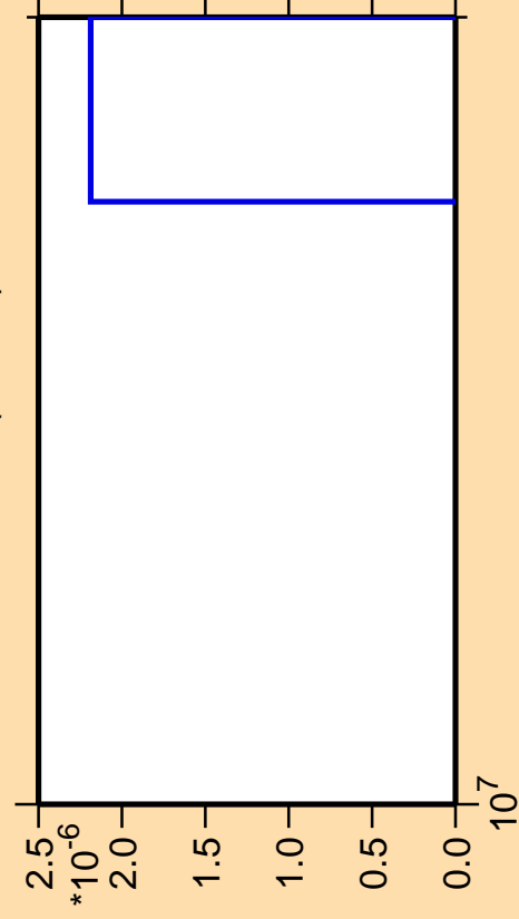
\Delta\sigma/\sigma vs. E for ^{162}\text{Sm} (mt 11)
