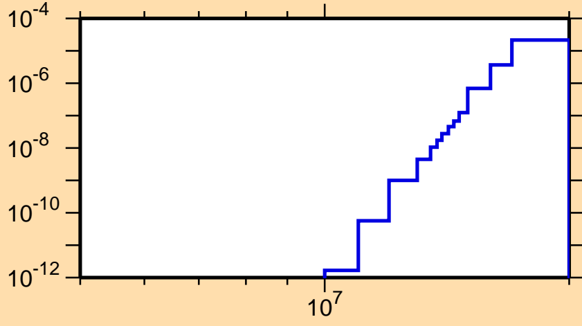
\sigma vs. E for ^{162}\text{Sm}(n,n\alpha)
