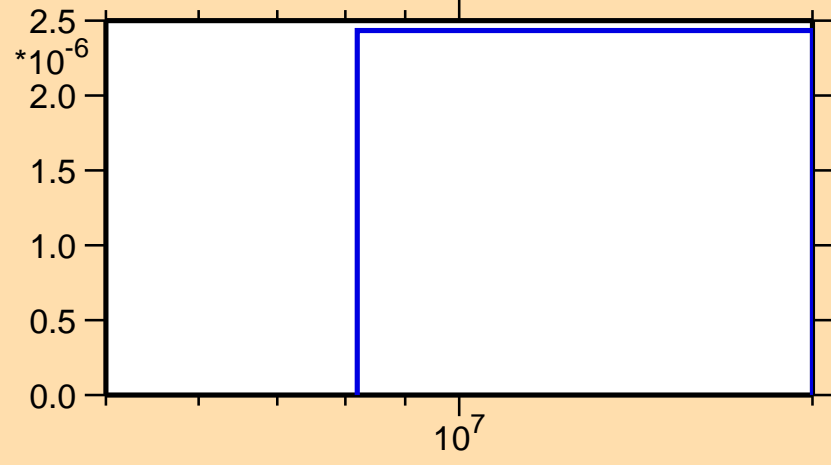
\sigma vs. E for ^{162}\text{Sm}(n,t)
