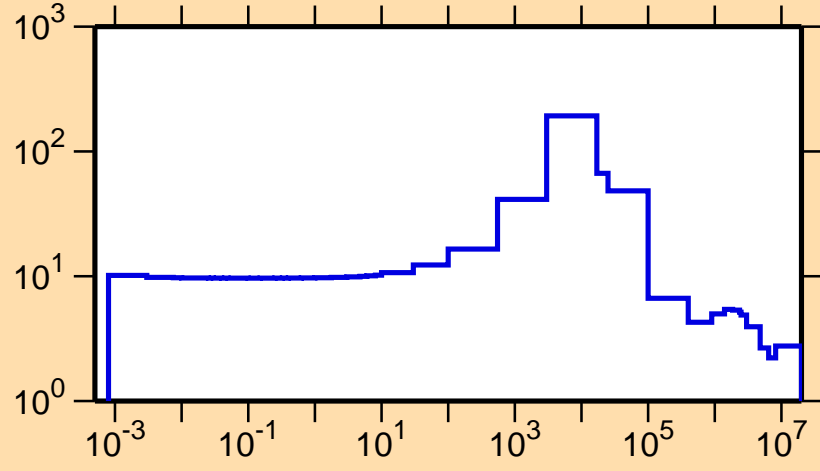
\sigma vs. E for ^{162}\text{Sm}(n,\text{el.})
