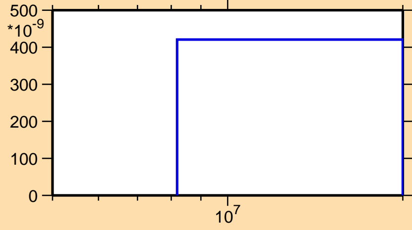
\sigma vs. E for ^{162}\text{Sm}(n,n\alpha)
