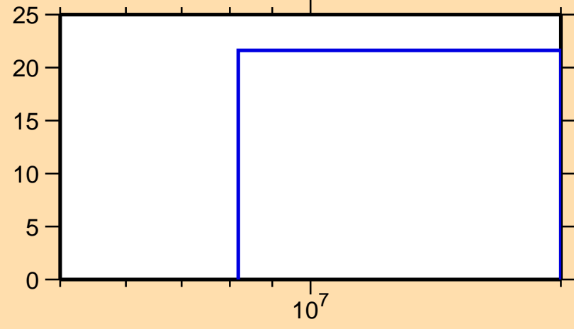
\Delta\sigma/\sigma vs. E for ^{162}\text{Sm}(n,el.)
