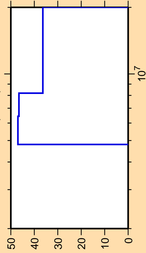
\Delta\sigma/\sigma vs. E for ^{162}\text{Sm}(n,2n)
