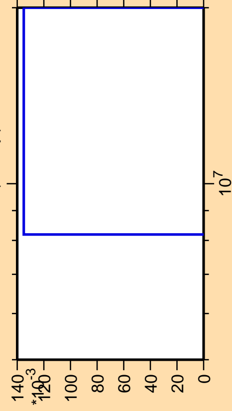
\Delta\sigma/\sigma vs. E for ^{162}\text{Sm}(n,2np)
