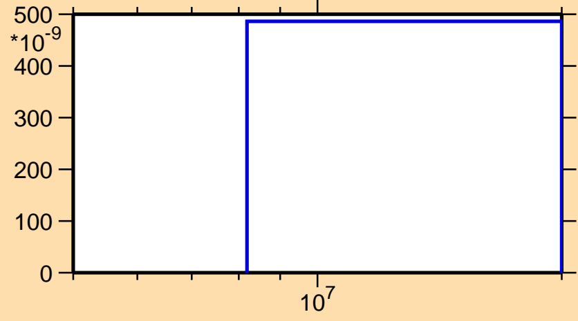
\sigma vs. E for ^{162}\text{Sm}(n,np)
