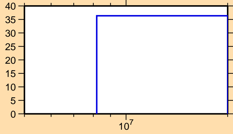
\Delta\sigma/\sigma vs. E for ^{162}\text{Sm}(n,2n)
