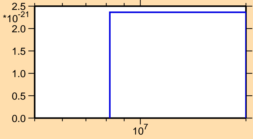
\sigma vs. E for ^{162}\text{Sm}(\text{mt } 11)
