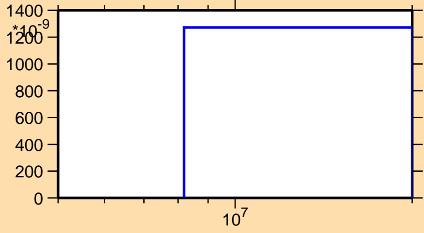
\sigma vs. E for ^{162}\text{Sm}(n,d)
