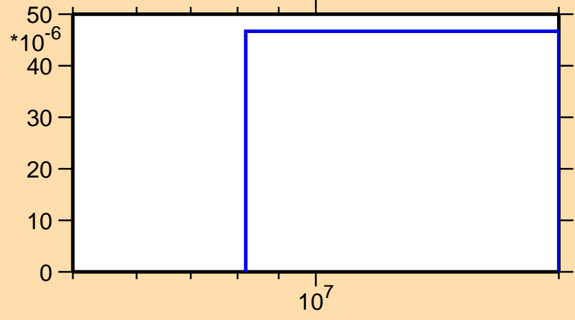
\sigma vs. E for ^{162}\text{Sm}(n,p)
