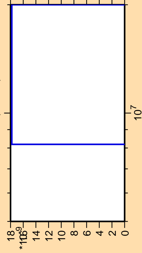
\Delta\sigma/\sigma vs. E for ^{162}\text{Sm}(\text{mt } 11)
