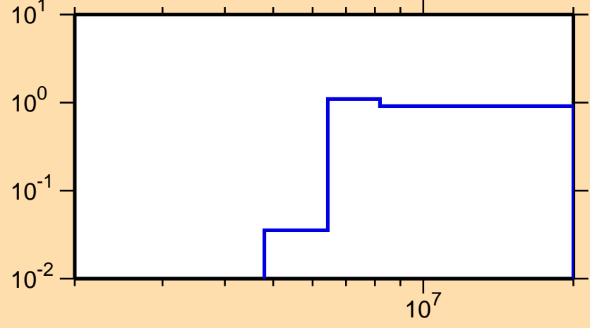
\sigma vs. E for ^{162}\text{Sm}(n,2n)
