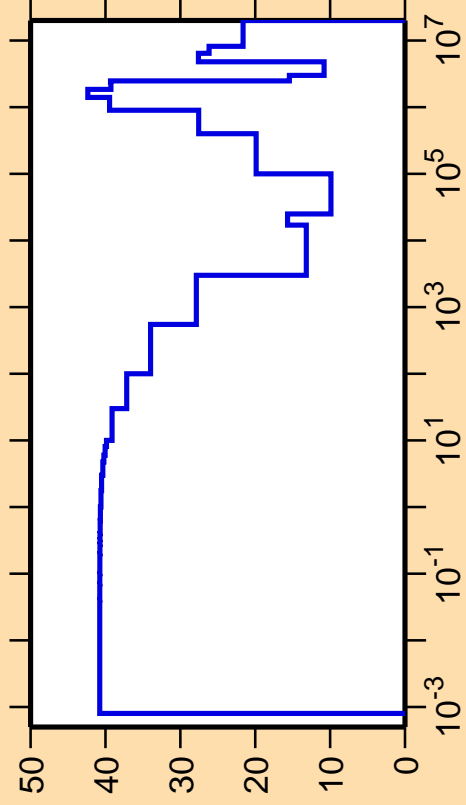
\Delta\sigma/\sigma vs. E for ^{162}\text{Sm}(n,\text{el.})
