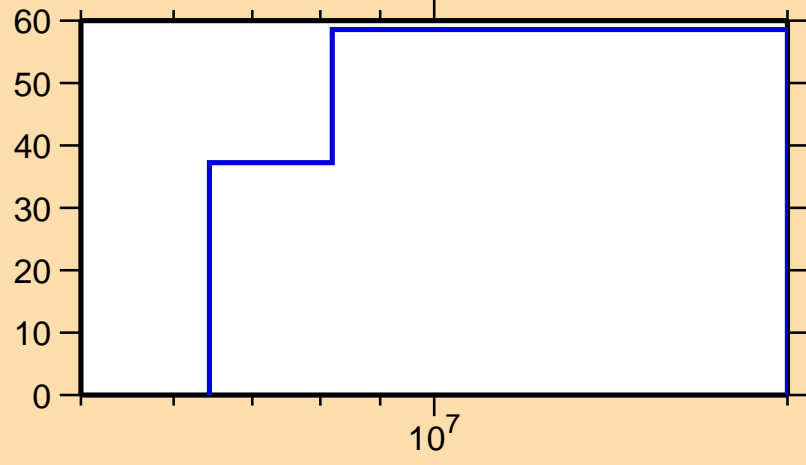
\Delta\sigma/\sigma vs. E for ^{162}\text{Sm}(n,ncont.)
