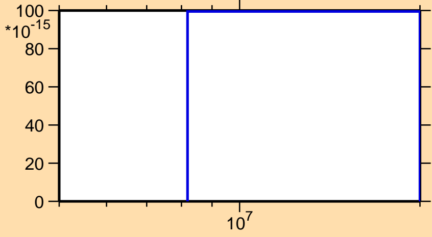
\sigma vs. E for ^{162}\text{Sm}(n,2np)
