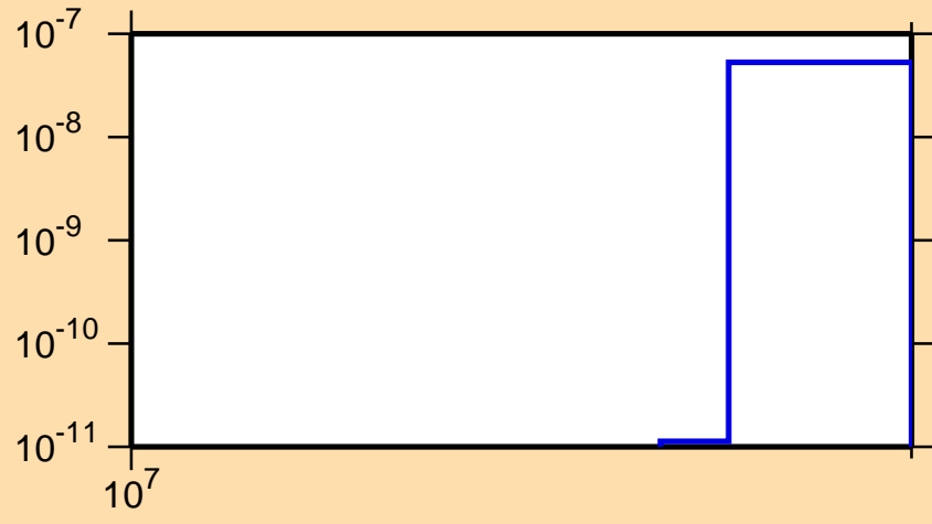
\sigma vs. E for ^{163}\text{Sm}(n,\text{nd})
