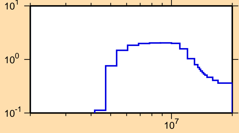
\sigma vs. E for ^{163}\text{Sm}(n,2n)
