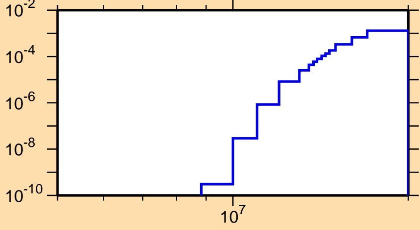
\sigma vs. E for ^{163}\text{Sm}(n,p)
