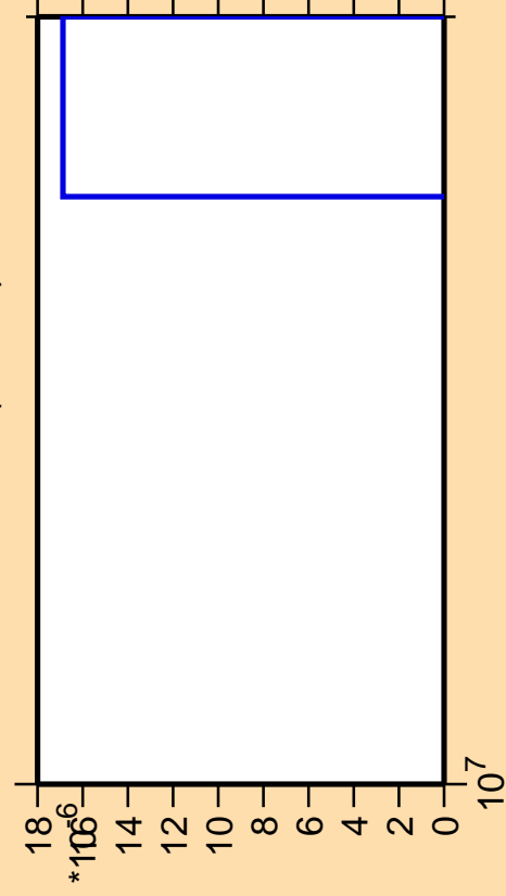
\Delta\sigma/\sigma vs. E for ^{163}\text{Sm} (mt 11)
