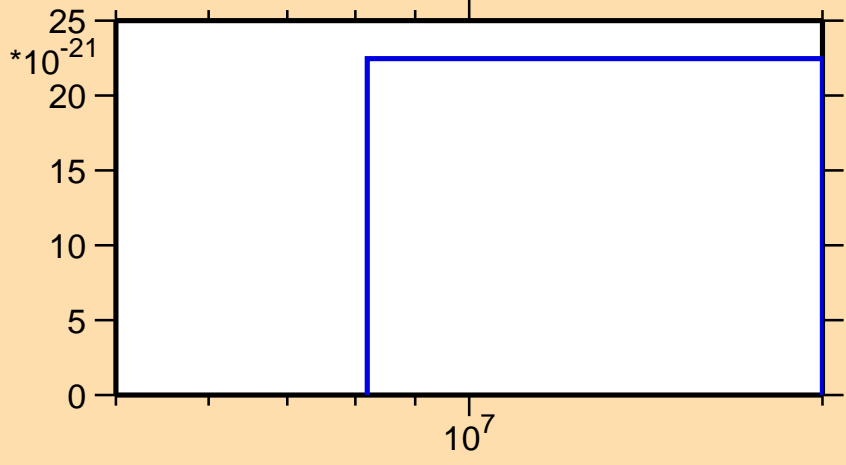
\sigma vs. E for ^{163}\text{Sm}(\text{mt } 11)
