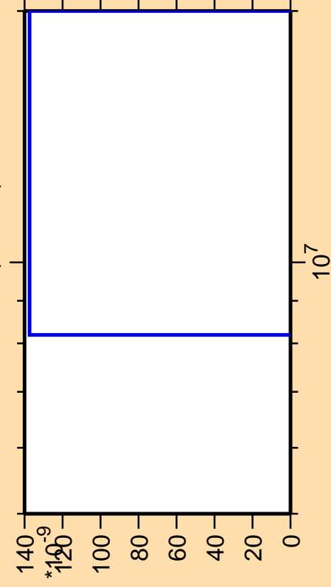
\Delta\sigma/\sigma vs. E for ^{163}\text{Sm}(\text{mt } 11)
