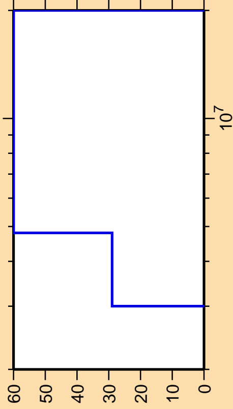
\Delta\sigma/\sigma vs. E for ^{163}\text{Sm}(n,n\text{cont.})
