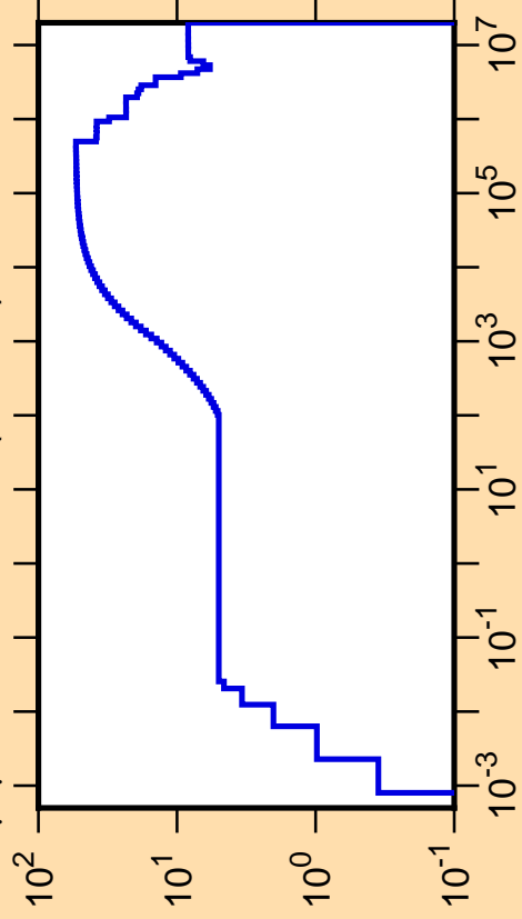
\Delta\mu/\mu vs. E for ^{139}\text{Tb}(\text{mt251})
