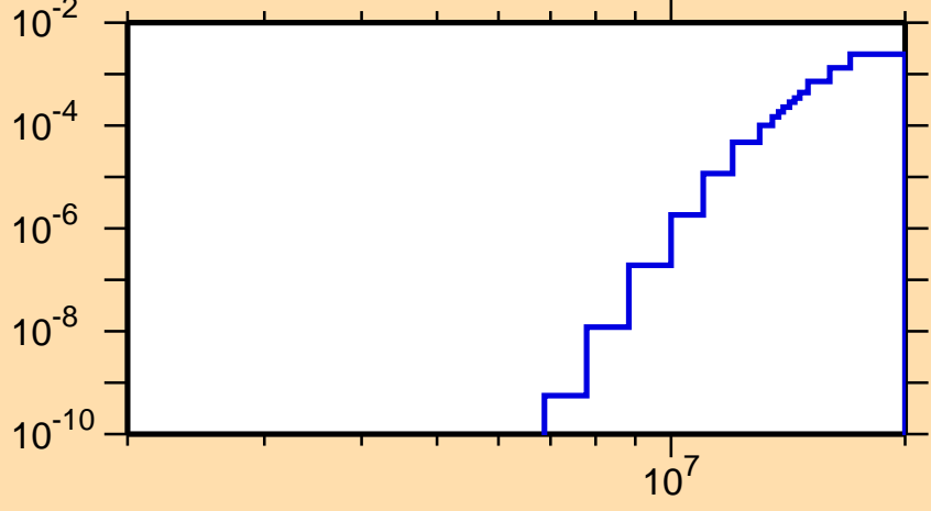
\sigma vs. E for ^{139}\text{Tb}(\text{mt } 45)
