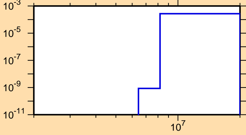
\sigma vs. E for ^{139}\text{Tb} (mt 45)
