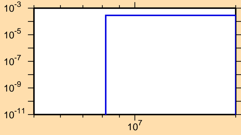
\sigma vs. E for ^{139}\text{Tb}(n,t)
