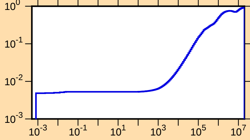
\mu vs. E for ^{140}\text{Tb}(\text{mt251})
