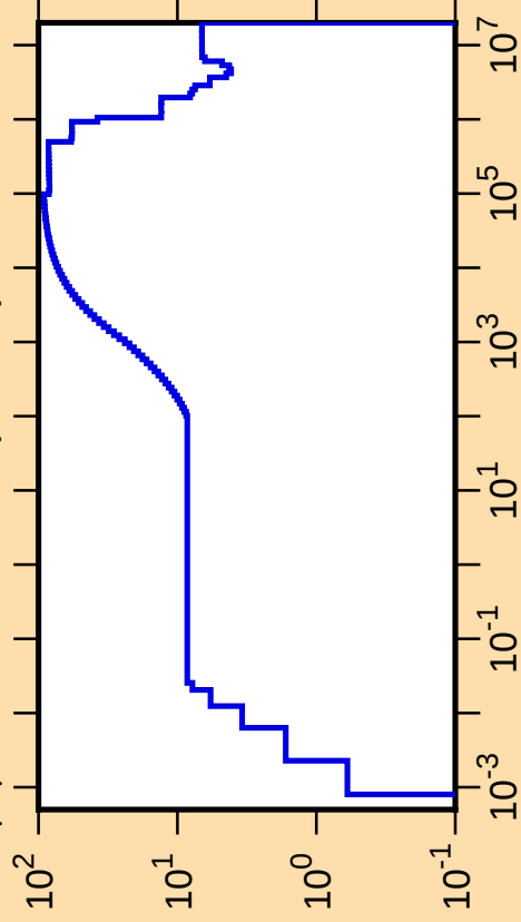
\Delta\mu/\mu vs. E for ^{140}\text{Tb}(\text{mt251})
