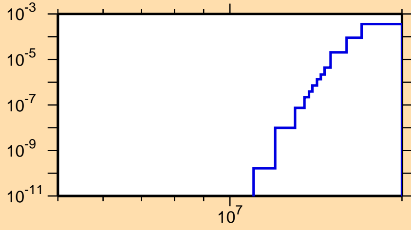
\sigma vs. E for ^{140}\text{Tb}(n,\text{pt})
