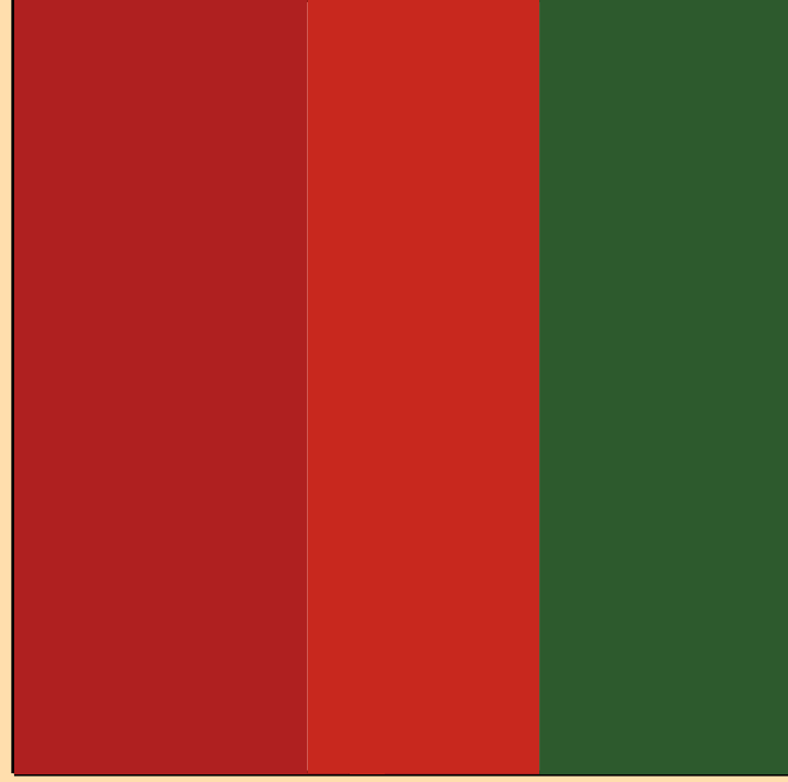
\Delta\sigma/\sigma vs. E for ^{140}\text{Tb}(n,2n)
