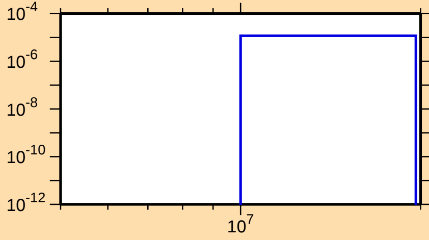
\sigma vs. E for ^{140}\text{Tb}(n,\text{pt})
