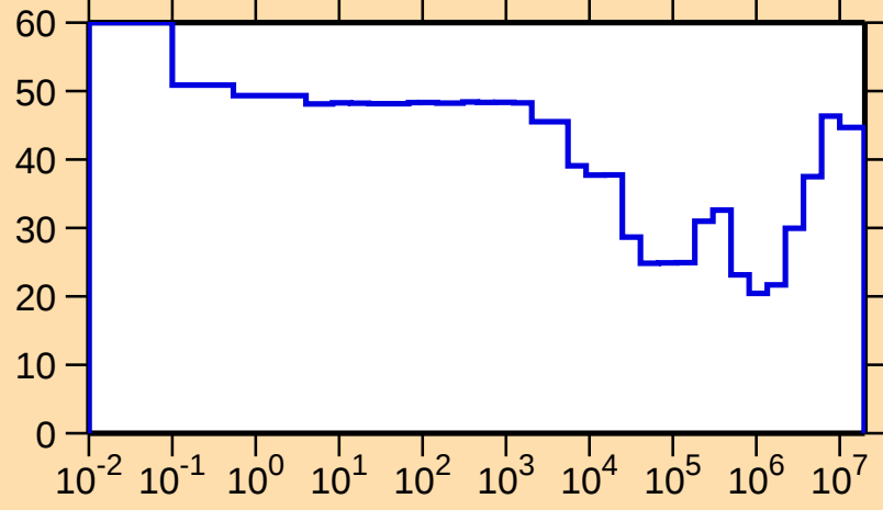
\Delta\sigma/\sigma vs. E for ^{140}\text{Tb}(n,p)
