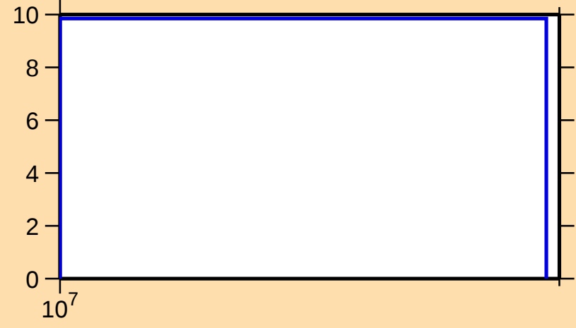
\Delta\sigma/\sigma vs. E for ^{140}\text{Tb}(n,\text{nonel.})
