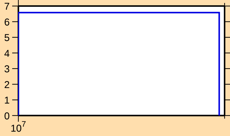
\Delta\sigma/\sigma vs. E for ^{140}\text{Tb}(n,\text{el.})
