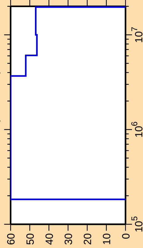
\Delta\sigma/\sigma vs. E for ^{140}\text{Tb}(n,\text{ncont.})
