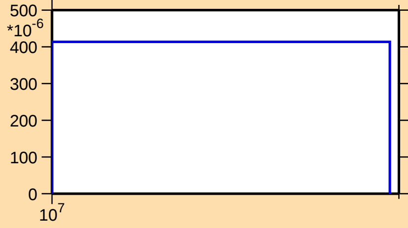
\sigma vs. E for ^{140}\text{Tb}(n,2n)
