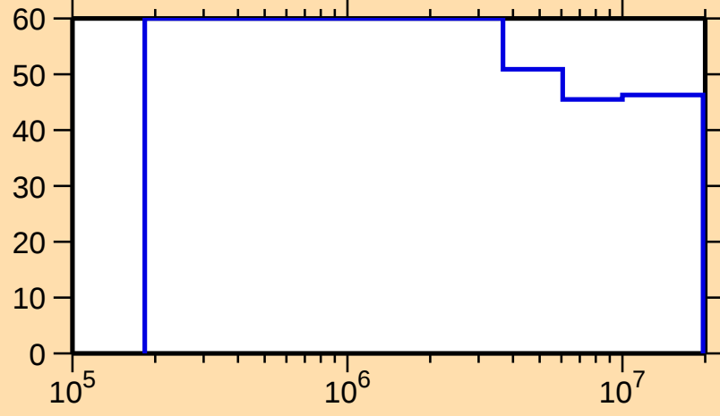
\Delta\sigma/\sigma vs. E for ^{140}\text{Tb}(n,\text{inel.})
