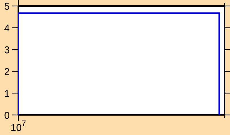
\Delta\sigma/\sigma vs. E for ^{140}\text{Tb}(n,\text{tot.})
