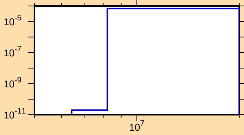
\sigma vs. E for ^{140}\text{Tb}(\text{mt } 45)
