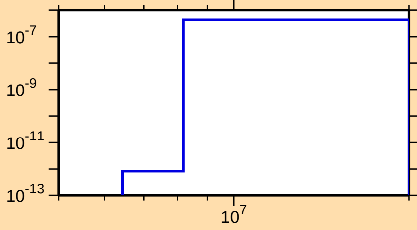
\sigma vs. E for ^{140}\text{Tb}(\text{mt117})
