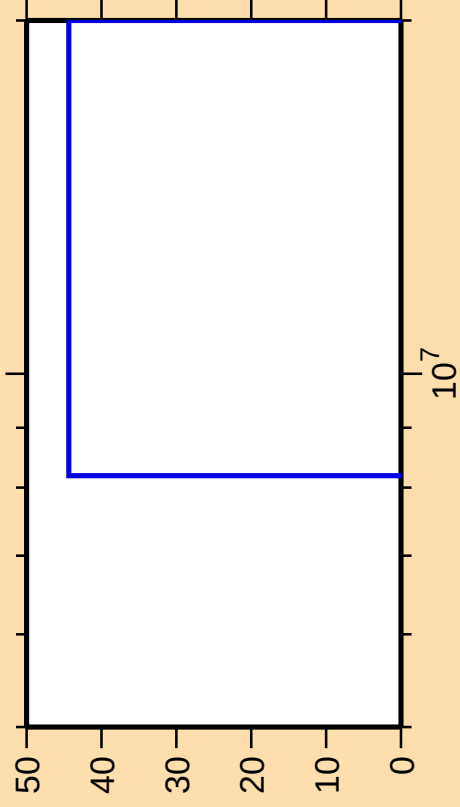
\Delta\sigma/\sigma vs. E for ^{140}\text{Tb}(n,n_1)
