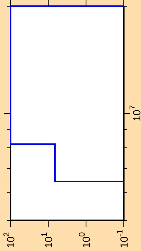
\Delta\sigma/\sigma vs. E for ^{140}\text{Tb}(\text{mt117})
