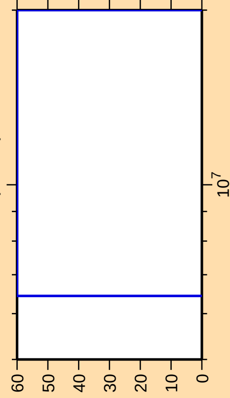
\Delta\sigma/\sigma vs. E for ^{140}\text{Tb}(\text{mt } 45)
