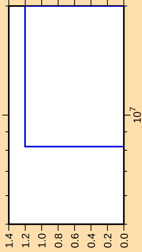
\Delta\sigma/\sigma vs. E for ^{140}\text{Tb}(n,\text{nt})
