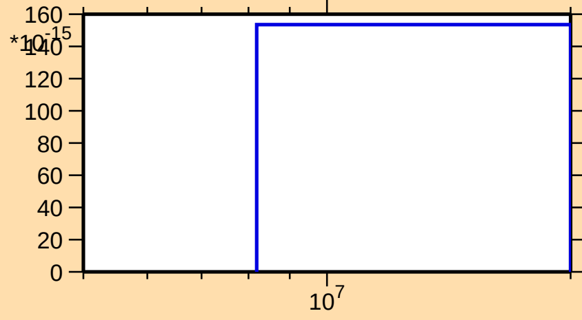
\sigma vs. E for ^{140}\text{Tb}(n,\text{nt})
