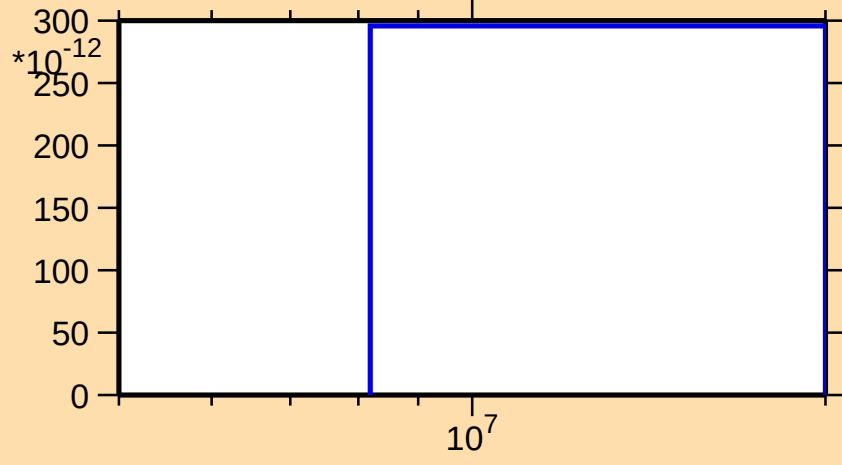
\sigma vs. E for ^{140}\text{Tb}(n,2n\alpha)
