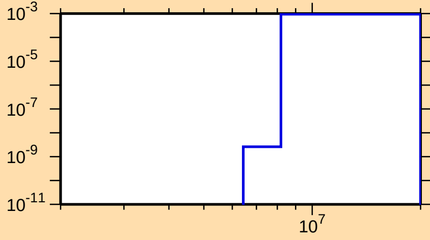
\sigma vs. E for ^{140}\text{Tb}(n,t)
