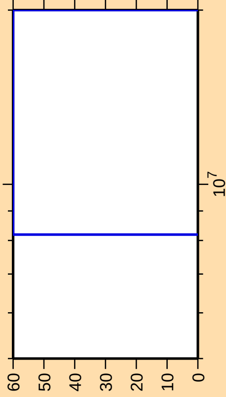
\Delta\sigma/\sigma vs. E for ^{140}\text{Tb}(n,2n\alpha)
