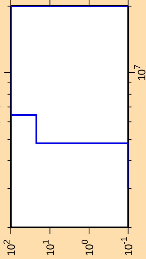
\Delta\sigma/\sigma vs. E for ^{140}\text{Tb}(n,t)
