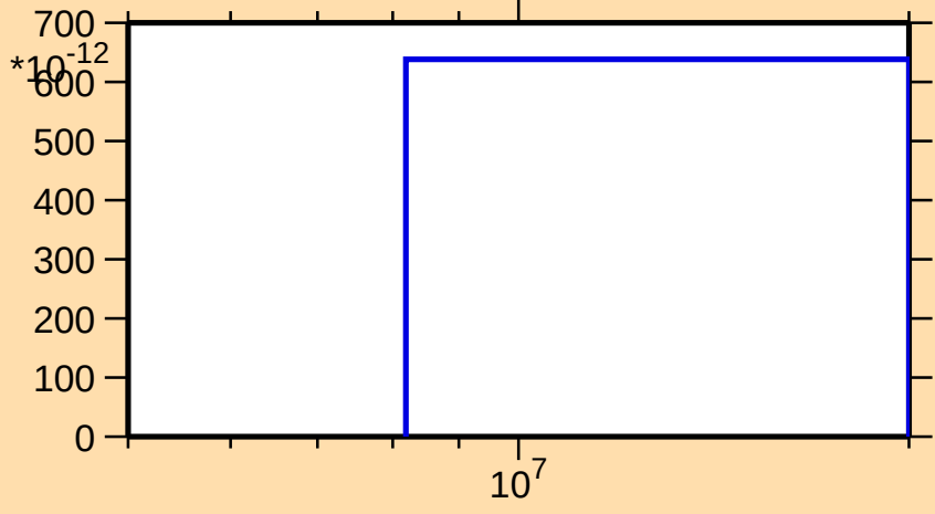
\sigma vs. E for ^{140}\text{Tb}(\text{mt } 34)
