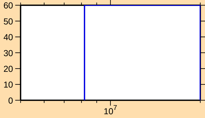
\Delta\sigma/\sigma vs. E for ^{140}\text{Tb}(n,2n)
