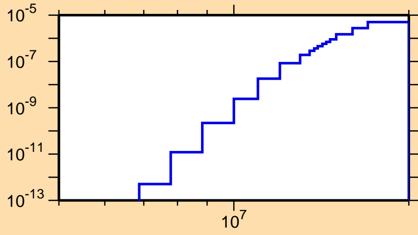
\sigma vs. E for ^{141}\text{Tb}(\text{mt117})
