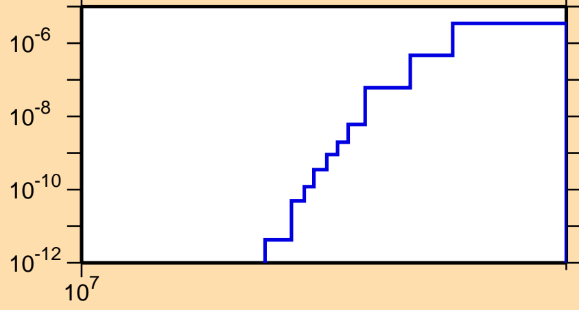
\sigma vs. E for ^{141}\text{Tb}(n,\text{nd})
