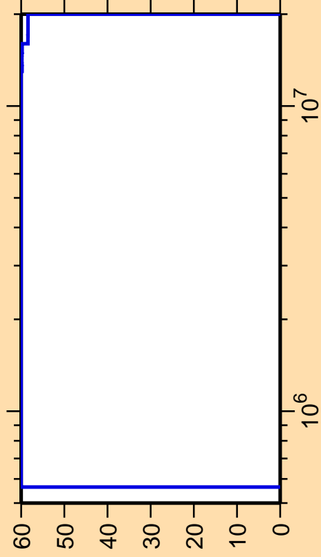
\Delta\sigma/\sigma vs. E for ^{141}\text{Tb}(n,n_2)
