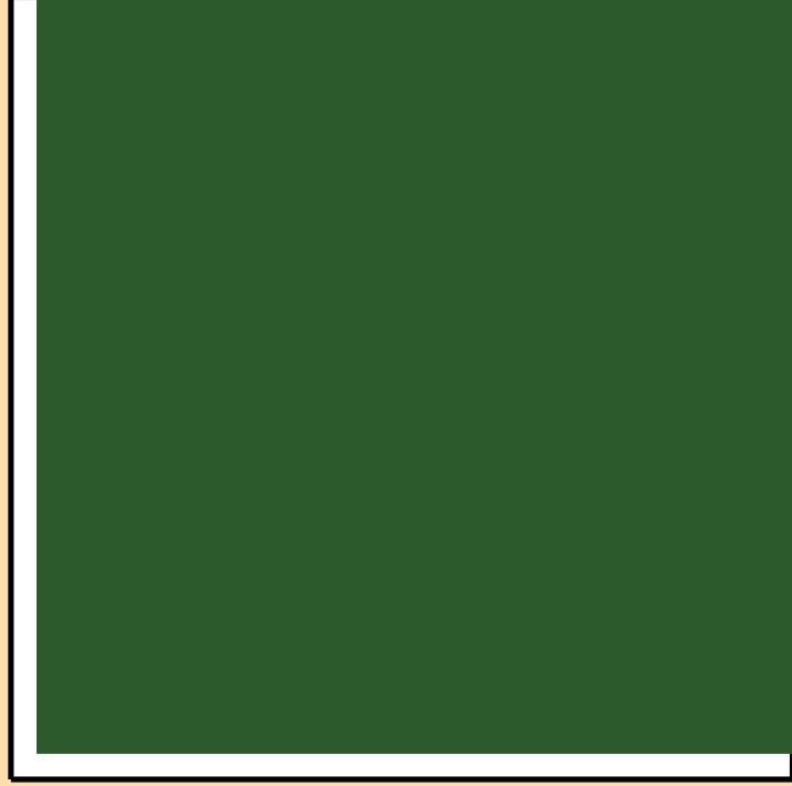
\sigma vs. E for ^{141}\text{Tb}(n,n_2)
