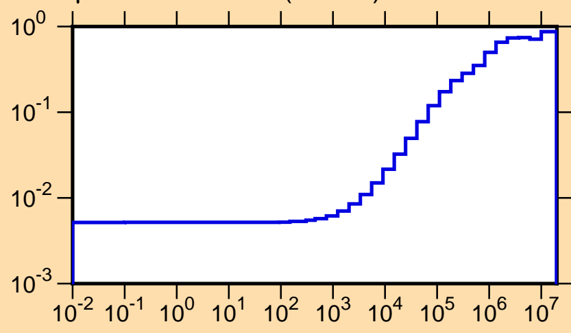
\mu vs. E for ^{141}\text{Tb}(\text{mt251})
