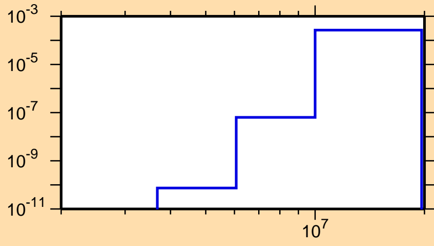
\sigma vs. E for ^{141}\text{Tb}(n,\text{He3})
