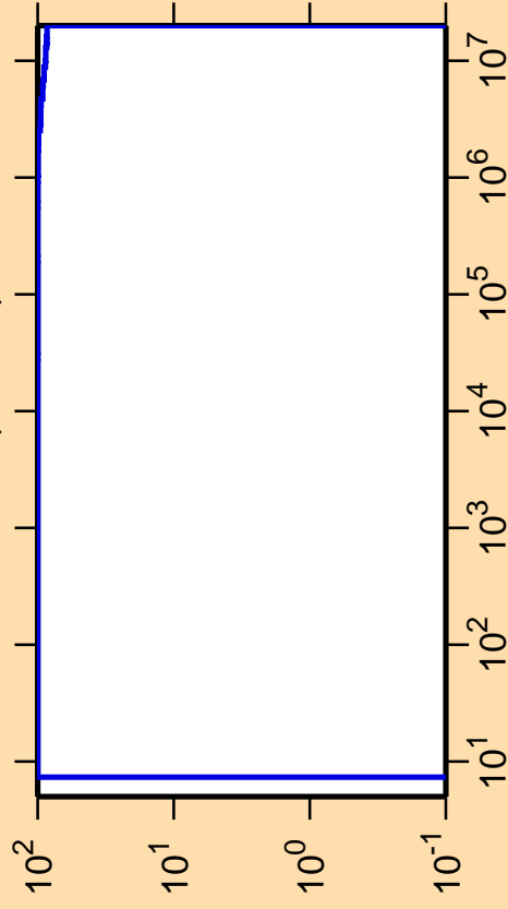
\Delta\sigma/\sigma vs. E for ^{141}\text{Tb}(n,\text{inel.})
