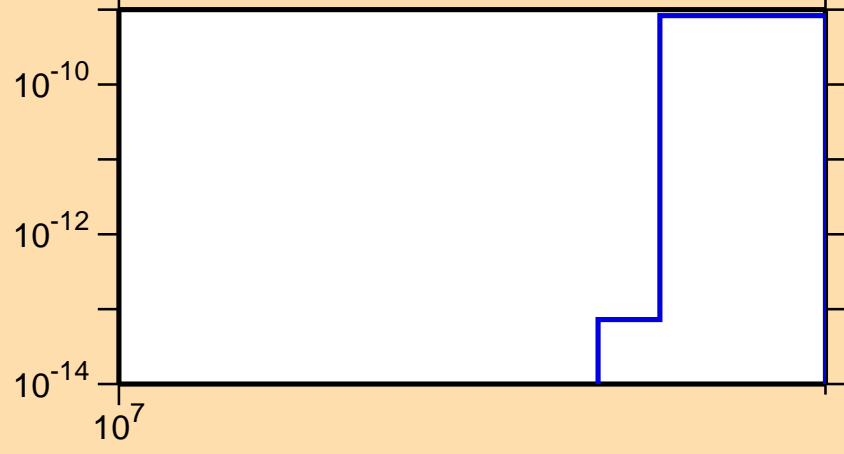
\sigma vs. E for ^{141}\text{Tb}(n,nt)
