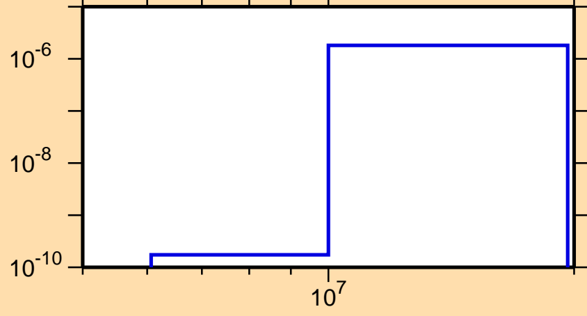
\sigma vs. E for ^{141}\text{Tb}(\text{mt117})
