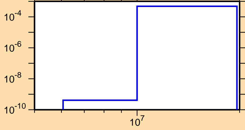
\sigma vs. E for ^{141}\text{Tb}(n,t)
