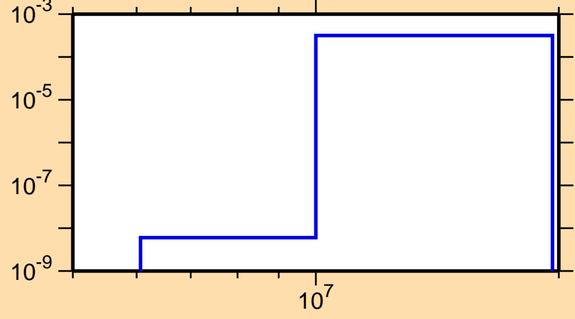
\sigma vs. E for ^{141}\text{Tb}(\text{mt } 45)
