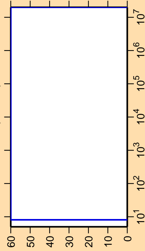
\Delta\sigma/\sigma vs. E for ^{141}\text{Tb}(n,\text{inel.})
