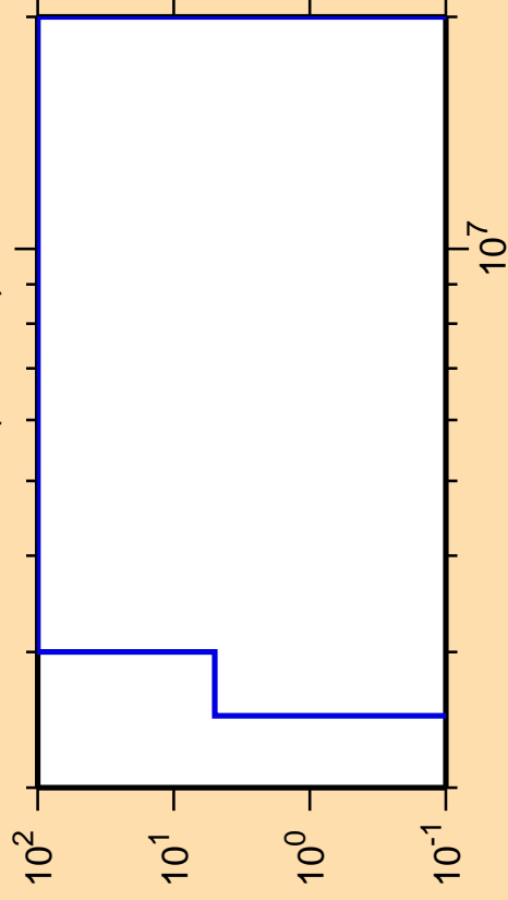
\Delta\sigma/\sigma vs. E for ^{141}\text{Tb}(n,\text{He3})
