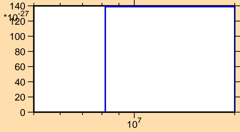
\sigma vs. E for ^{141}\text{Tb}(\text{mt } 11)
