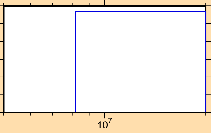
\sigma vs. E for ^{141}\text{Tb}(n,\text{nd})
