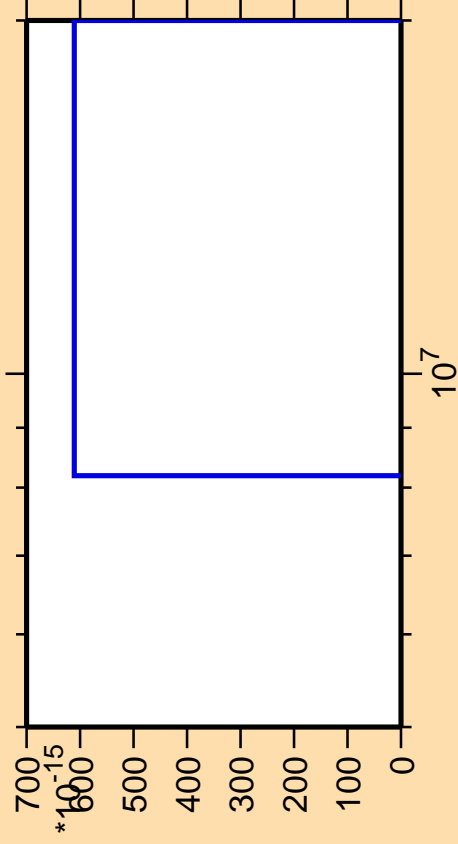
\Delta\sigma/\sigma vs. E for ^{141}\text{Tb}(\text{mt } 11)
