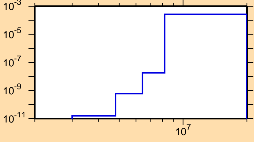
\sigma vs. E for ^{141}\text{Tb}(n,\text{He3})
