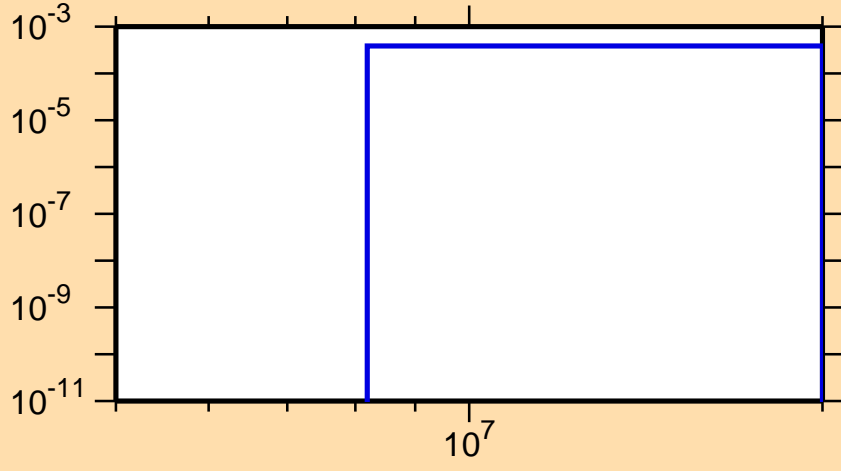
\sigma vs. E for ^{141}\text{Tb}(n,t)
