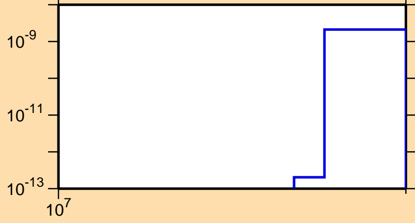
\sigma vs. E for ^{143}\text{Tb}(n,nt)
