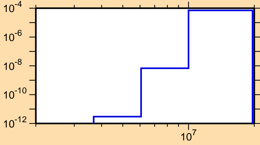
\sigma vs. E for ^{143}\text{Tb}(n,\text{He3})
