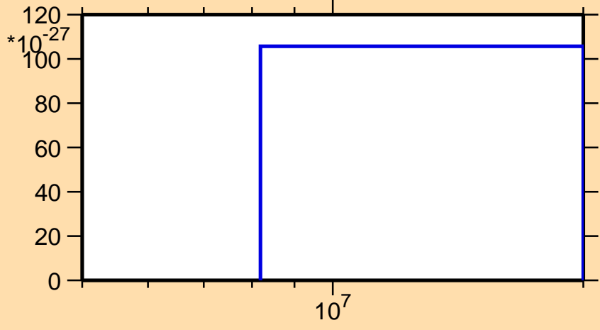
\sigma vs. E for ^{143}\text{Tb} (mt 11)
