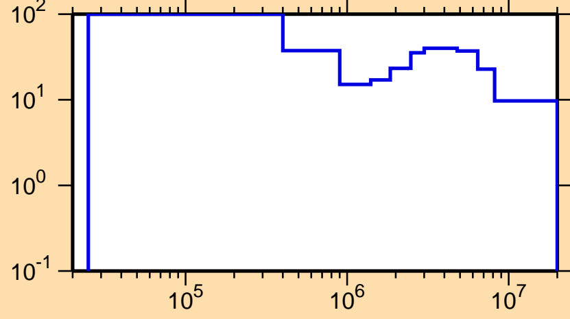
\Delta\sigma/\sigma vs. E for ^{143}\text{Tb}(n,\text{el.})
