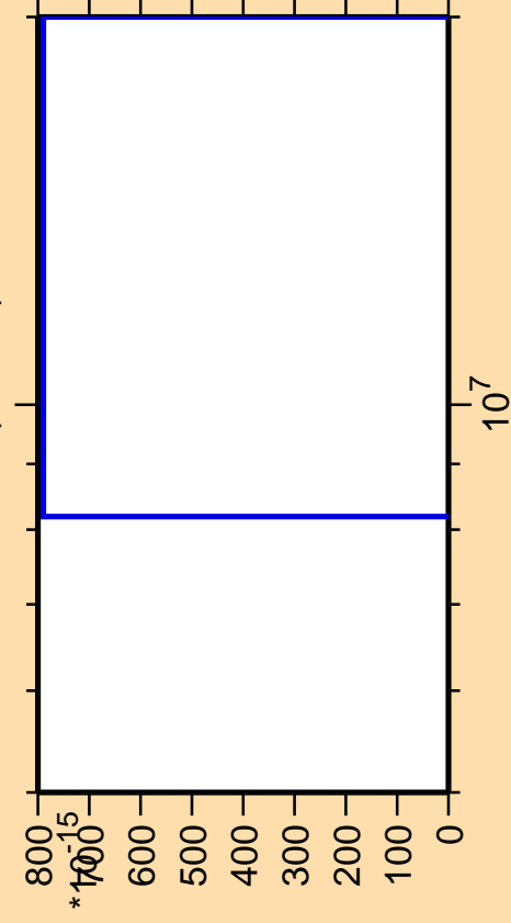
\Delta\sigma/\sigma vs. E for ^{143}\text{Tb} (mt 11)
