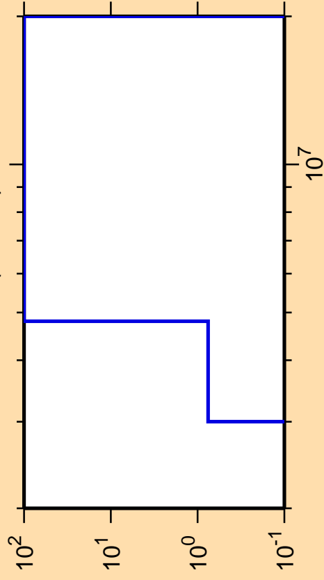
\Delta\sigma/\sigma vs. E for ^{143}\text{Tb}(n,\text{He3})
