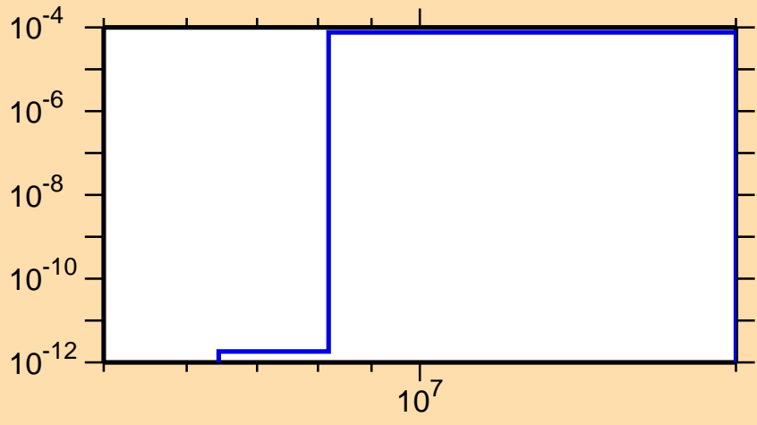
\sigma vs. E for ^{143}\text{Tb} (mt 45)
