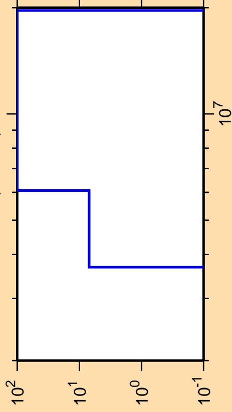
\Delta\sigma/\sigma vs. E for ^{144}\text{Tb}(n,\text{He3})
