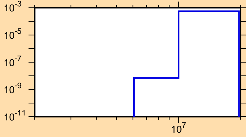
\sigma vs. E for ^{144}\text{Tb}(n,t)
