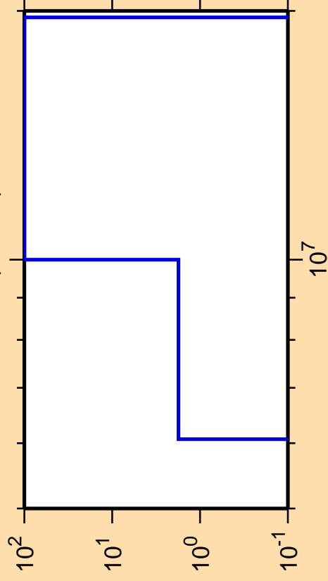
\Delta\sigma/\sigma vs. E for ^{144}\text{Tb}(\text{mt } 45)
