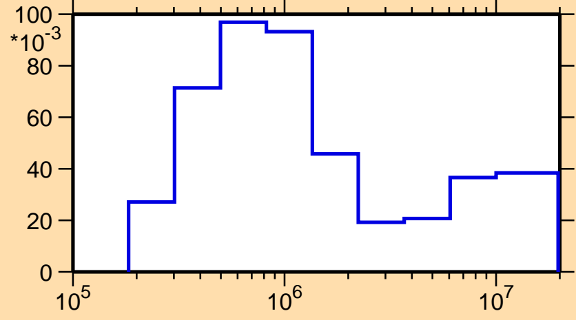
\sigma vs. E for ^{144}\text{Tb}(n,\text{inel.})
