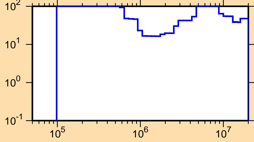
\Delta\sigma/\sigma vs. E for ^{144}\text{Tb}(n,\text{el.})
