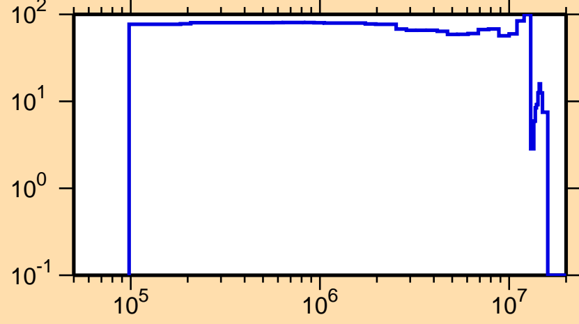
\Delta\sigma/\sigma vs. E for ^{144}\text{Tb}(n,n_1)
