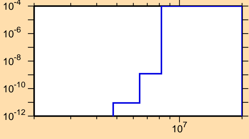
\sigma vs. E for ^{144}\text{Tb}(n,\text{He3})
