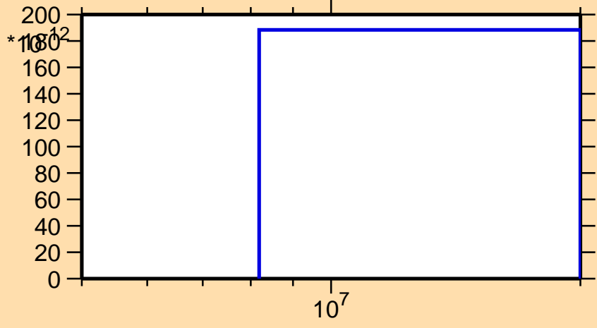
\sigma vs. E for ^{144}\text{Tb}(\text{mt } 34)
