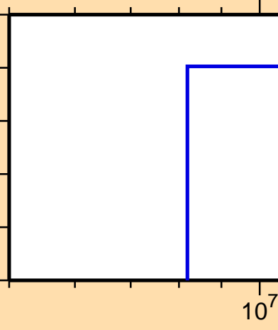
\sigma vs. E for ^{144}\text{Tb}(n,2n)
