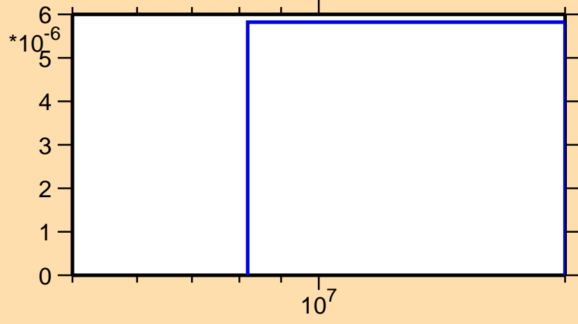
\sigma vs. E for ^{144}\text{Tb}(n,\text{pd})
