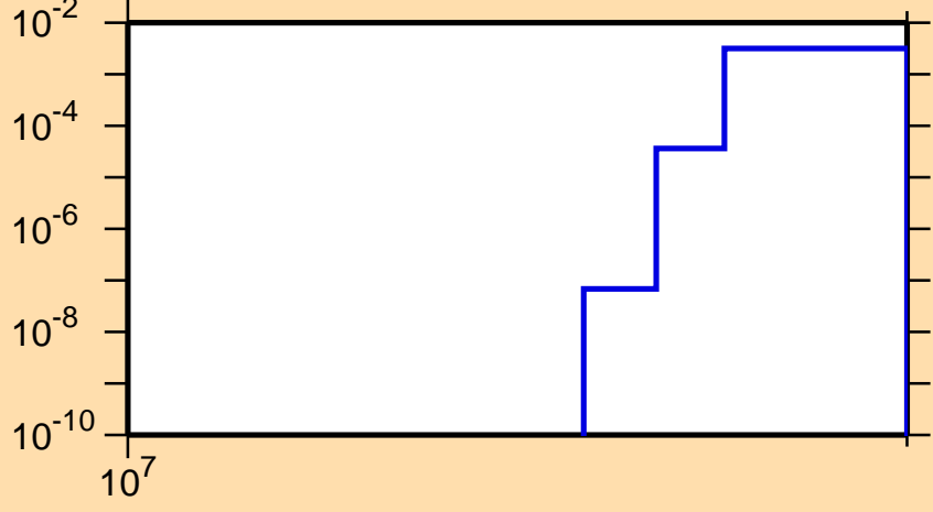
\sigma vs. E for ^{145}\text{Tb}(n,2np)
