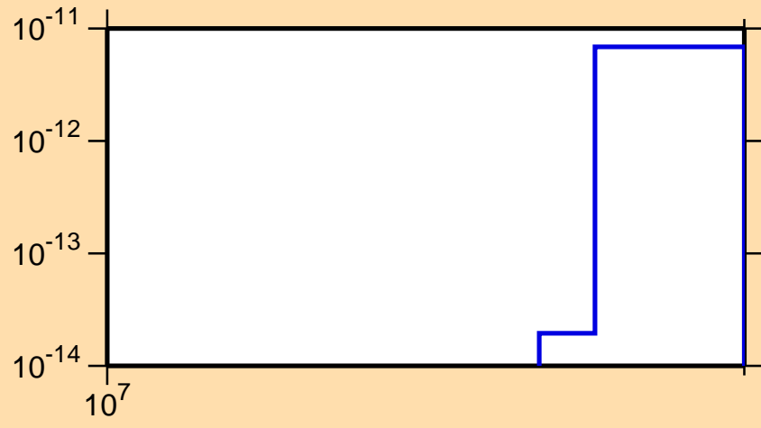
\sigma vs. E for ^{145}\text{Tb} (mt 34)
